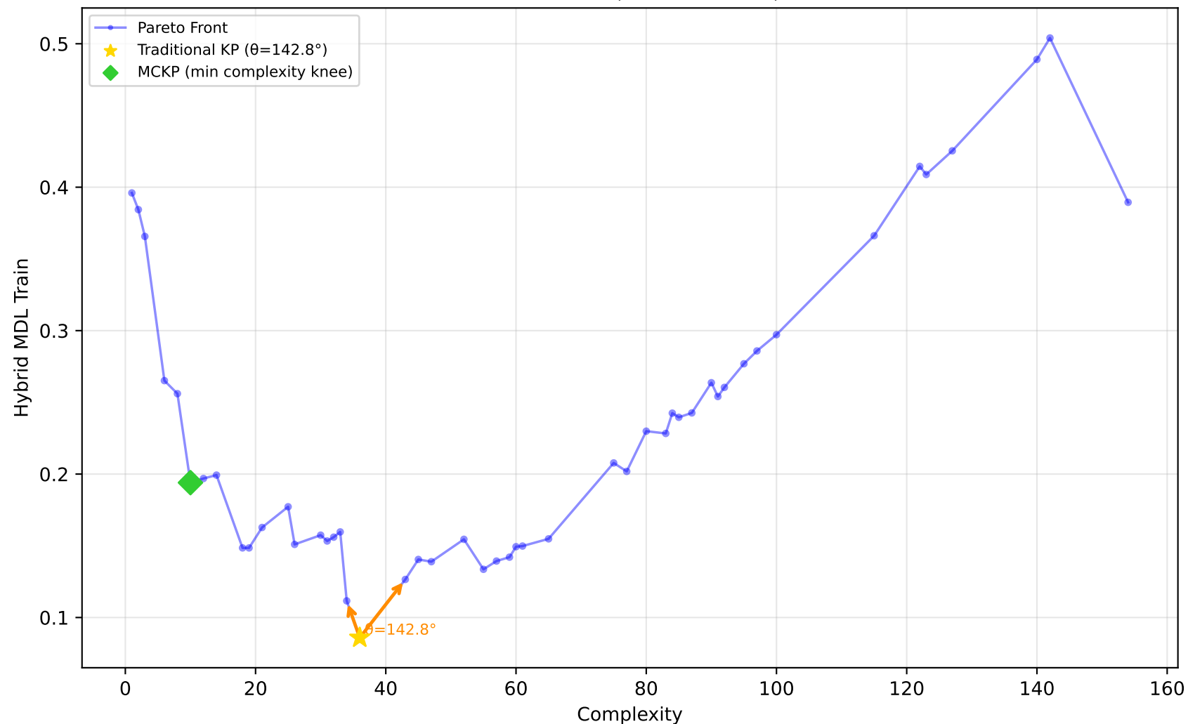
584_fri_c4_500_25 - Run 15 - SVP - Hybrid MDL Train \lambda_1=0.00, \lambda_2=0.00, \lambda_3=0.00 | Difficulty: 1.00 | Method: hmr
