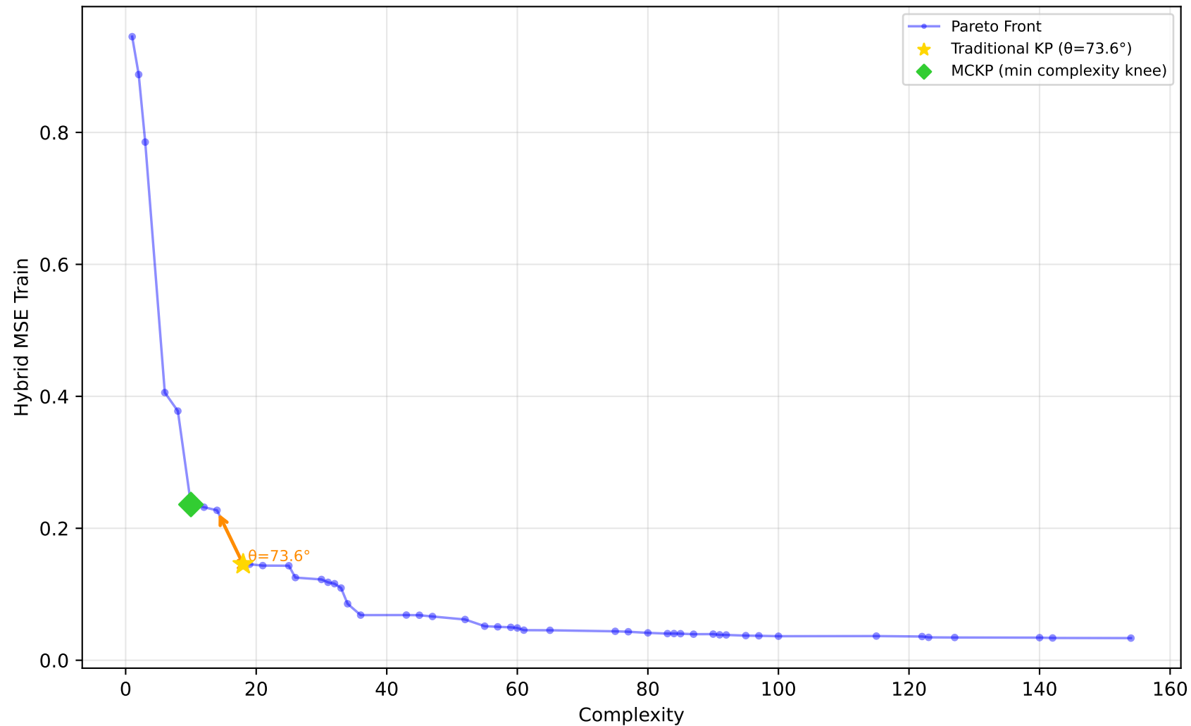
584_fri_c4_500_25 - Run 15 - SVP - Hybrid MSE Train \lambda_1=0.10, \lambda_2=0.40, \lambda_3=0.00 | Difficulty: 1.00 | Method: hmr
