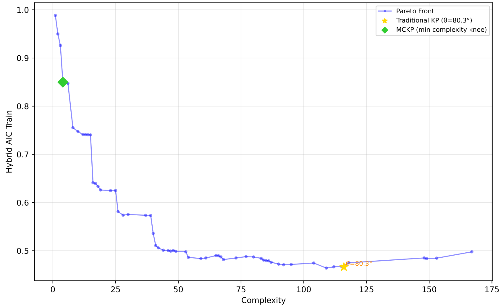
584_fri_c4_500_25 - Run 16 - MVP - Hybrid AIC Train \lambda_1=0.00, \lambda_2=0.00, \lambda_3=0.00 | Difficulty: 1.00 | Method: hmr
