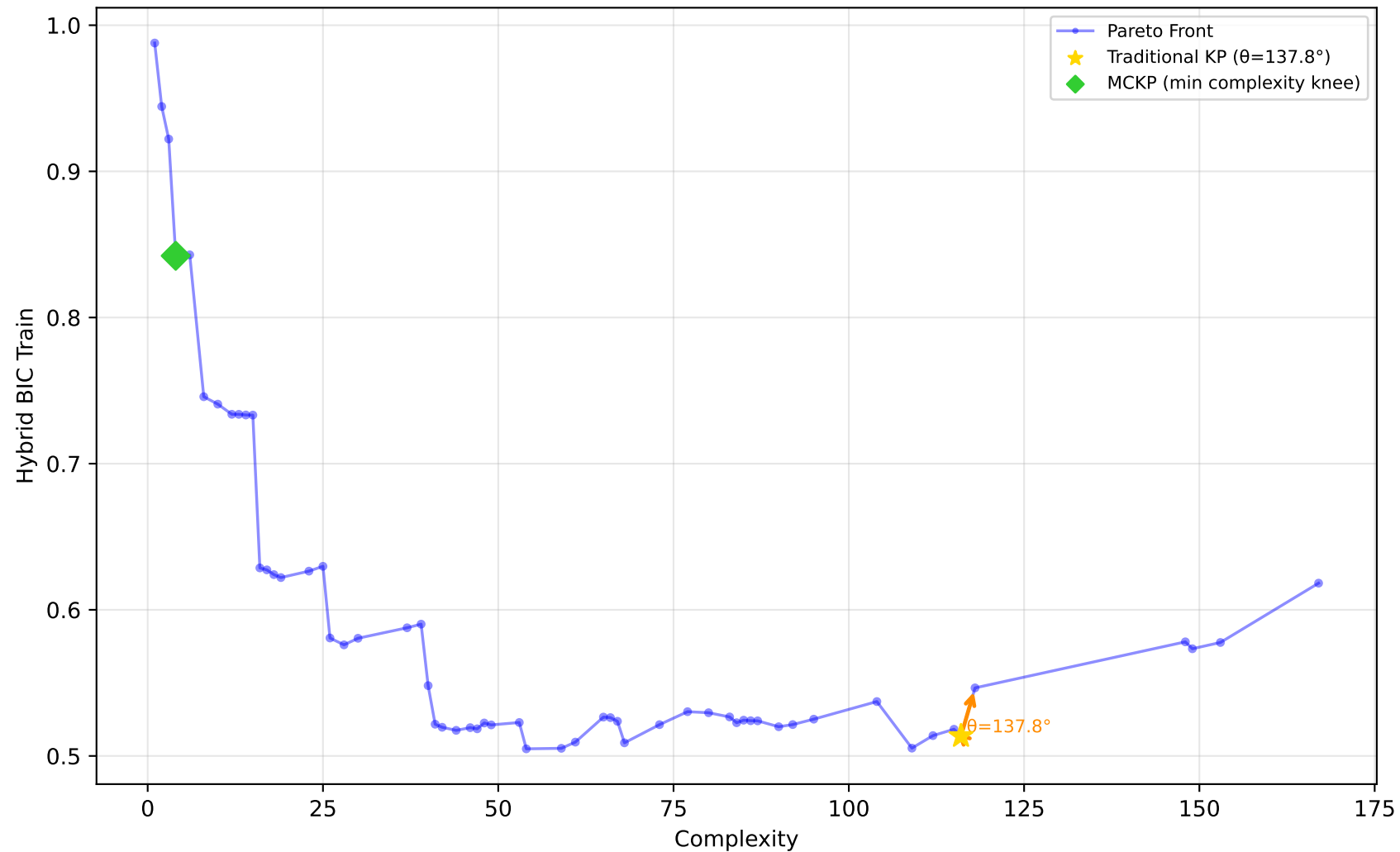
584_fri_c4_500_25 - Run 16 - MVP - Hybrid BIC Train \lambda_1=0.00, \lambda_2=0.00, \lambda_3=0.00 | Difficulty: 1.00 | Method: hmr
