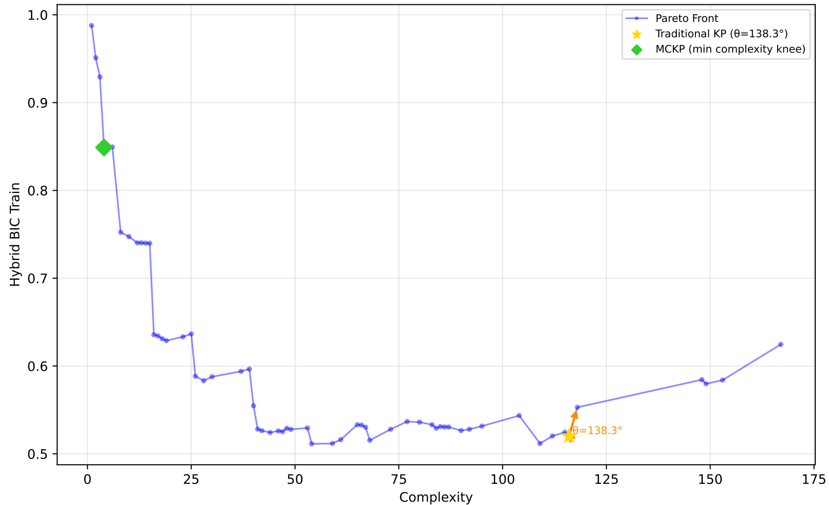
584_fri_c4_500_25 - Run 16 - MVP - Hybrid BIC Train \lambda_1=0.10, \lambda_2=0.00, \lambda_3=0.00 | Difficulty: 1.00 | Method: hmr
