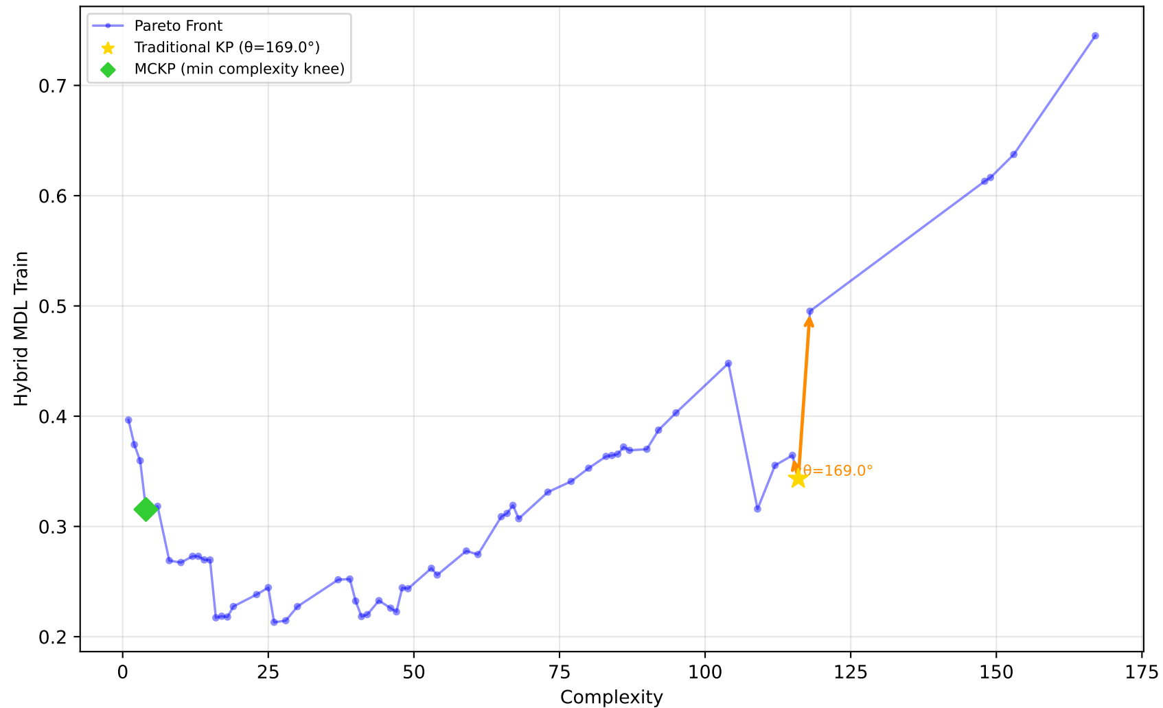
584_fri_c4_500_25 - Run 16 - MVP - Hybrid MDL Train \lambda_1=0.00, \lambda_2=0.00, \lambda_3=0.00 | Difficulty: 1.00 | Method: hmr
