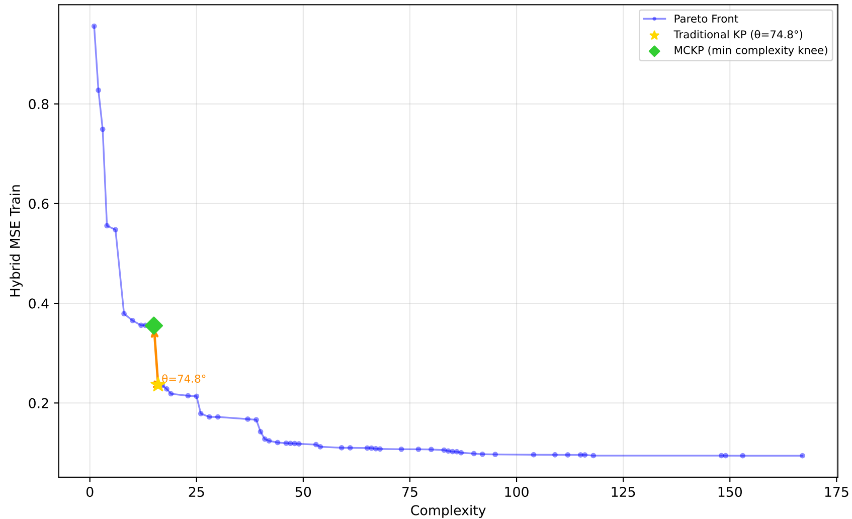
584_fri_c4_500_25 - Run 16 - MVP - Hybrid MSE Train \lambda_1=0.00, \lambda_2=0.00, \lambda_3=0.00 | Difficulty: 1.00 | Method: hmr
