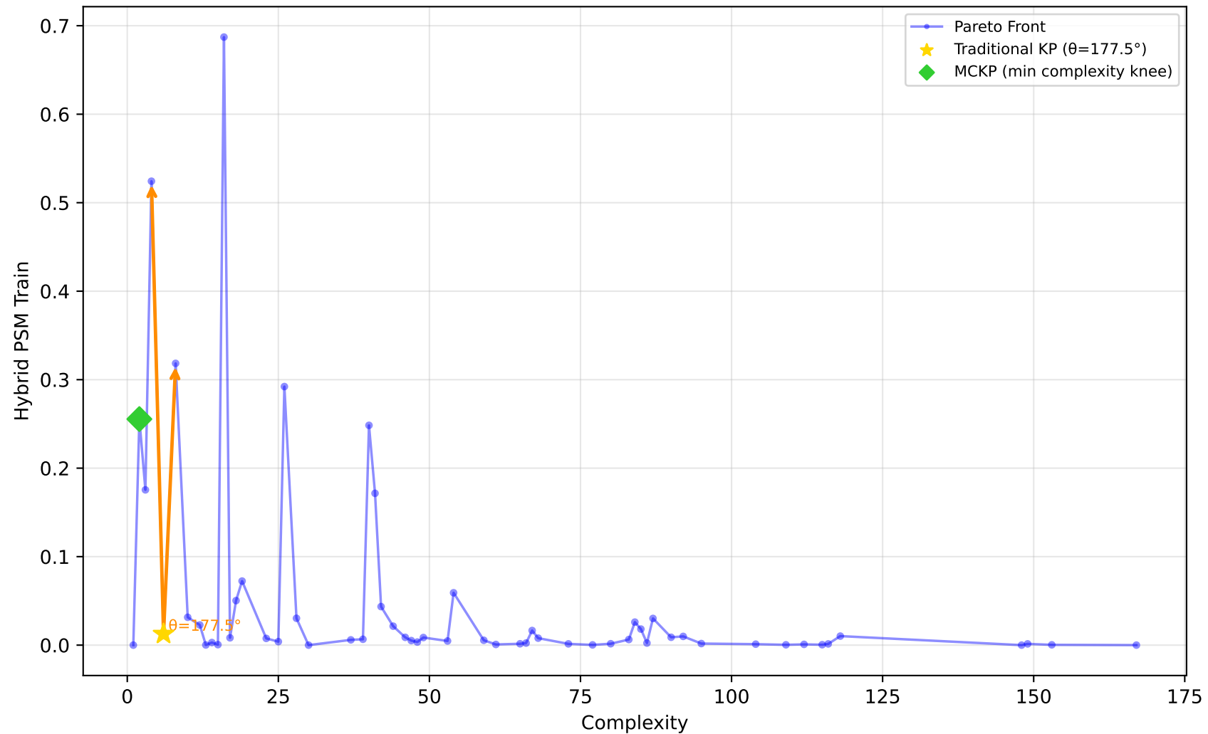
584_fri_c4_500_25 - Run 16 - MVP - Hybrid PSM Train \lambda_1=0.00, \lambda_2=0.00, \lambda_3=0.00 | Difficulty: 1.00 | Method: hmr
