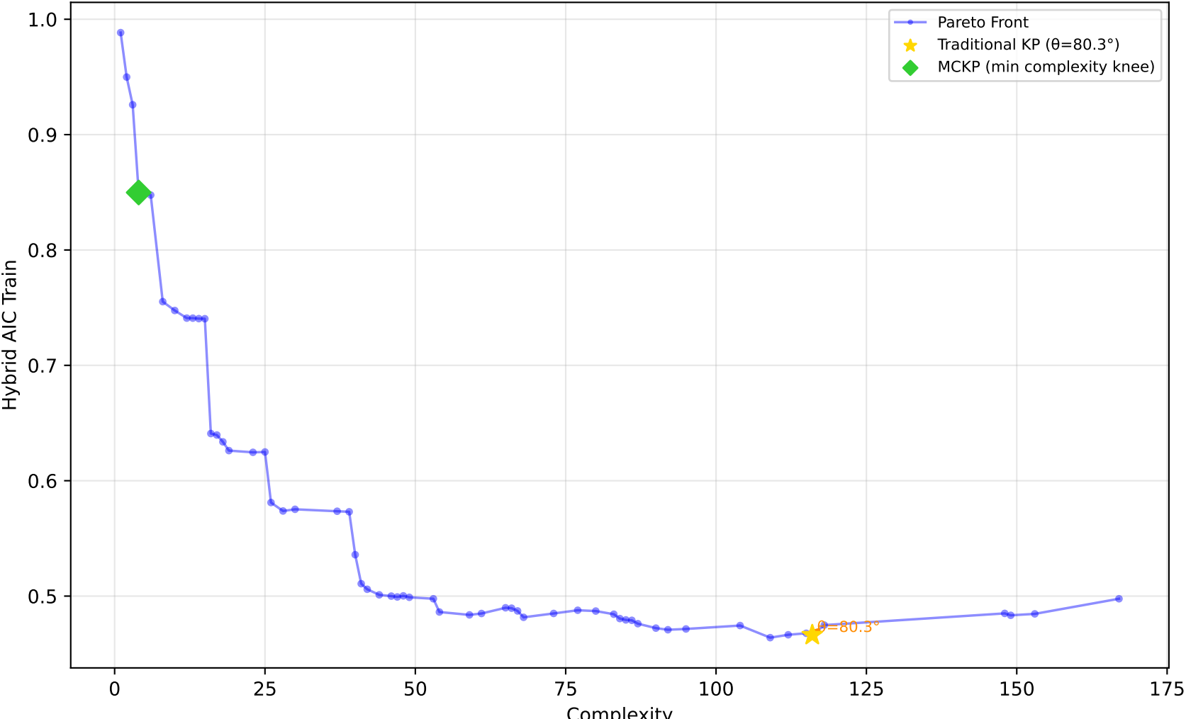
584_fri_c4_500_25 - Run 16 - SVP - Hybrid AIC Train \lambda_1=0.00 , \lambda_2=0.00 , \lambda_3=0.00 | Difficulty: 1.00 | Method: hmr
