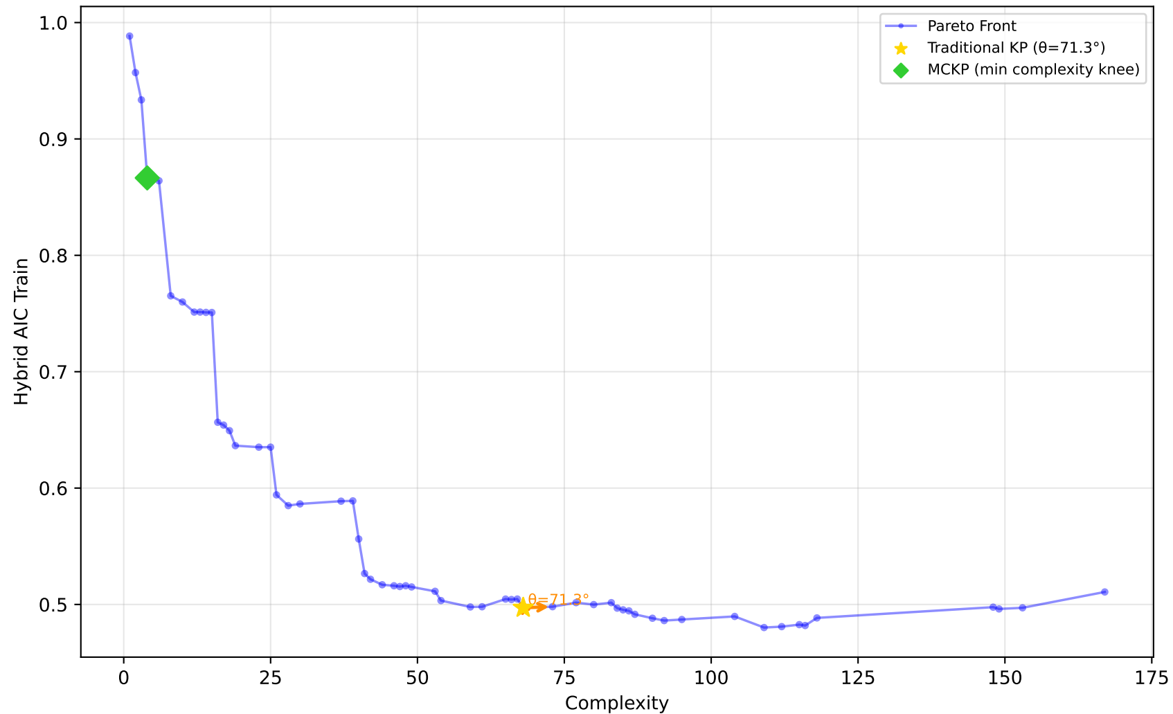
584_fri_c4_500_25 - Run 16 - SVP - Hybrid AIC Train \lambda_1=0.10, \lambda_2=0.40, \lambda_3=0.00 | Difficulty: 1.00 | Method: hmr
