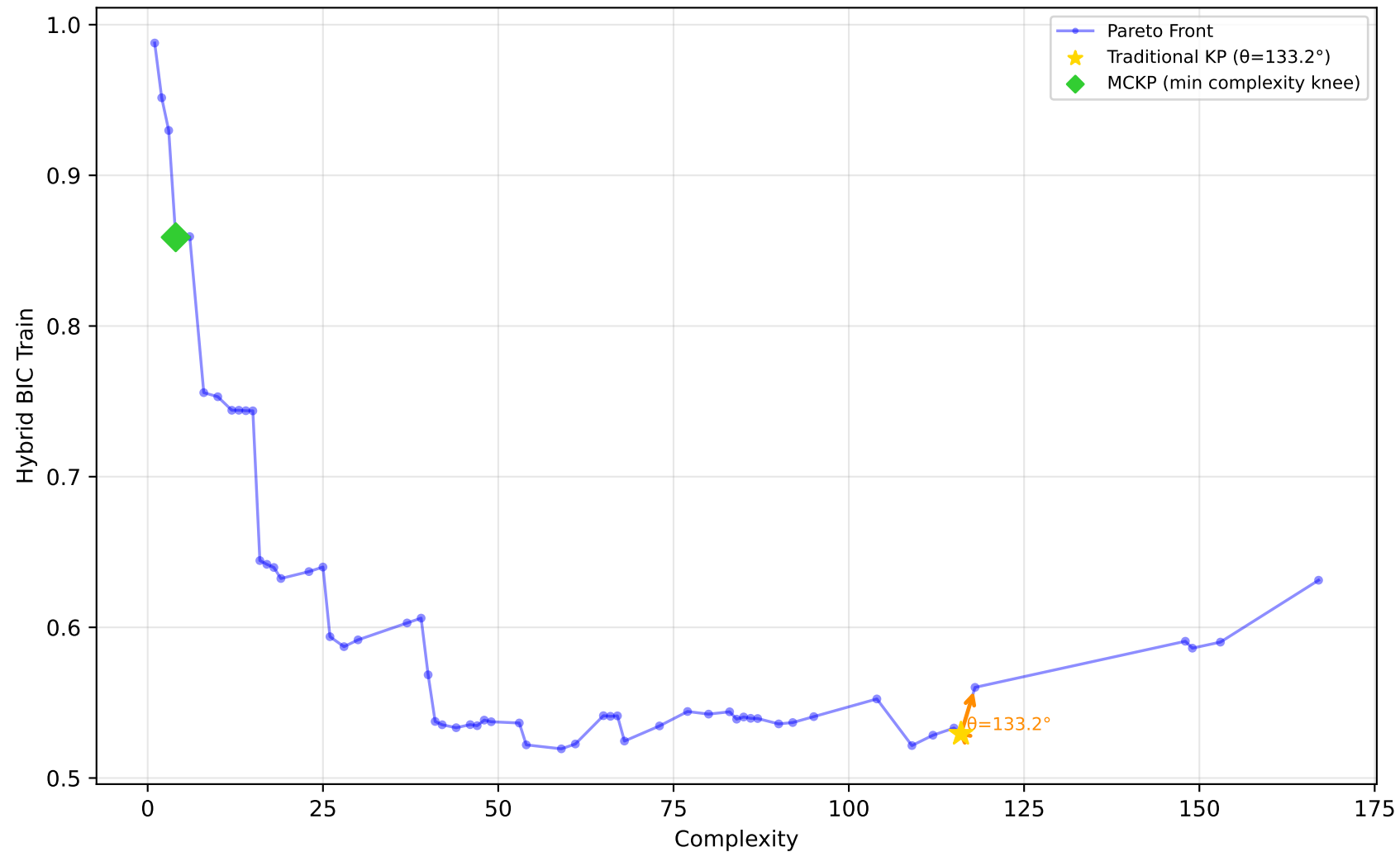
584_fri_c4_500_25 - Run 16 - SVP - Hybrid BIC Train \lambda_1=0.10, \lambda_2=0.40, \lambda_3=0.00 | Difficulty: 1.00 | Method: hmr
