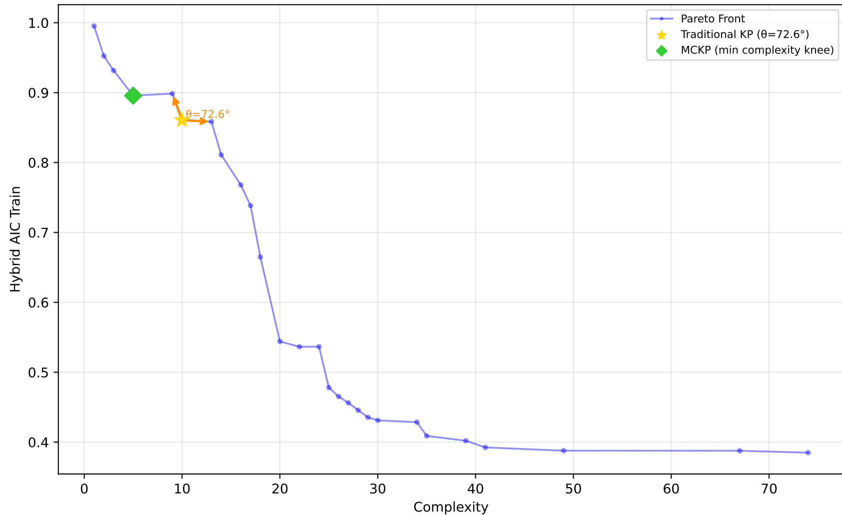
584_fri_c4_500_25 - Run 17 - MVP - Hybrid AIC Train \lambda_1=0.10, \lambda_2=0.00, \lambda_3=0.00 | Difficulty: 1.00 | Method: hmr
