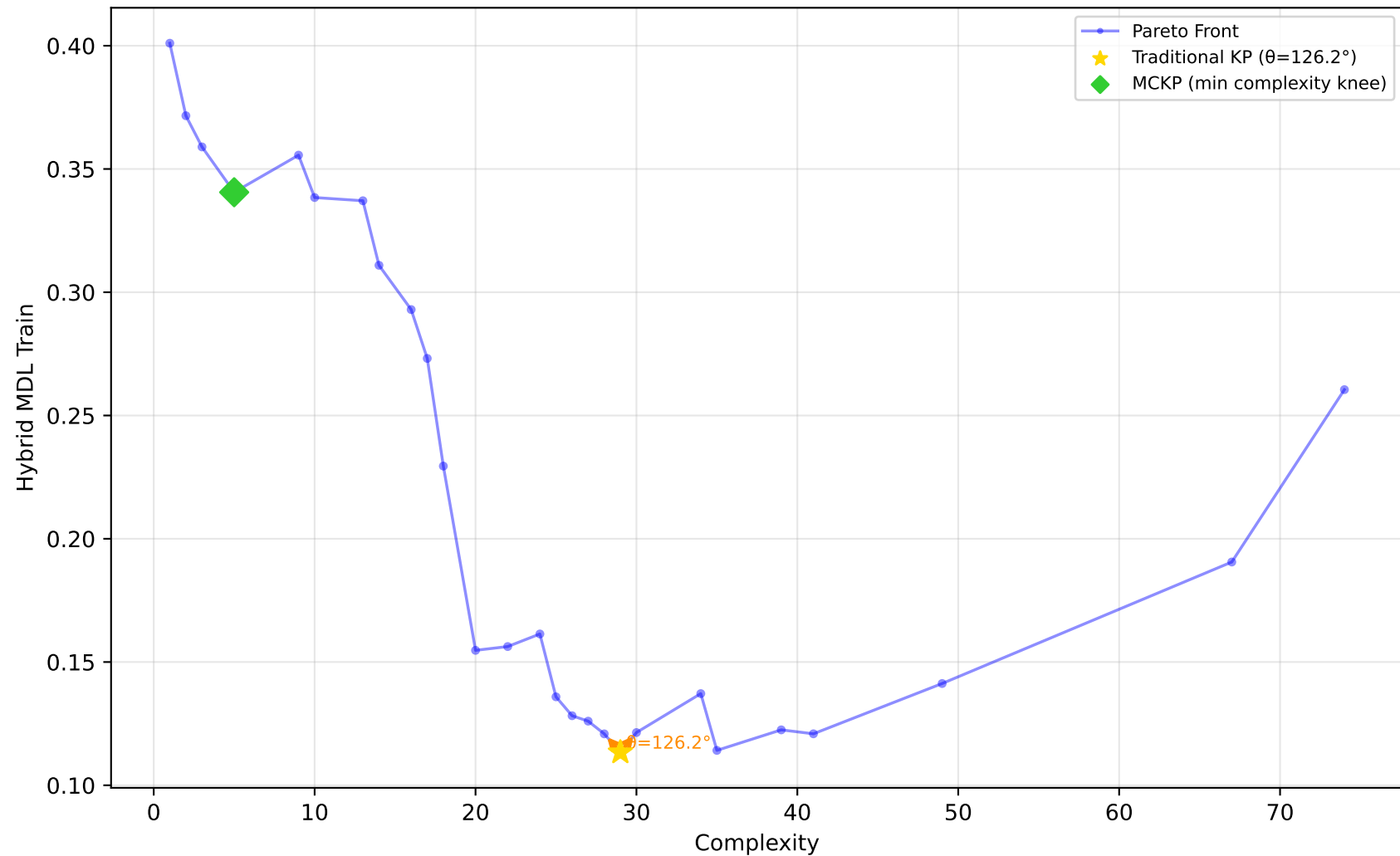
584_fri_c4_500_25 - Run 17 - MVP - Hybrid MDL Train \lambda_1=0.00 , \lambda_2=0.00 , \lambda_3=0.00 | Difficulty: 1.00 | Method: hmr
