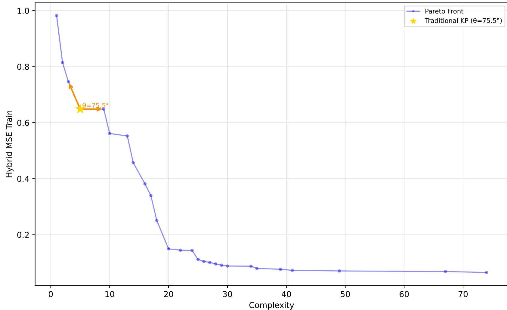
584_fri_c4_500_25 - Run 17 - MVP - Hybrid MSE Train \lambda_1=0.00, \lambda_2=0.00, \lambda_3=0.00 | Difficulty: 1.00 | Method: hmr
