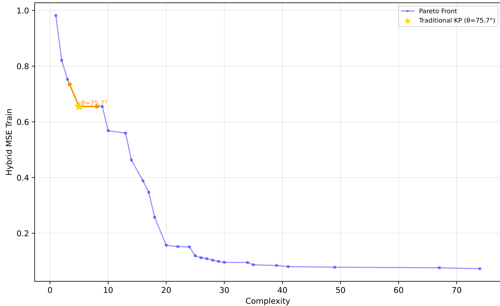
584_fri_c4_500_25 - Run 17 - MVP - Hybrid MSE Train \lambda_1=0.10, \bar{\lambda}_2=0.00, \bar{\lambda}_3=0.00 | Difficulty: 1.00 | Method: hmr
