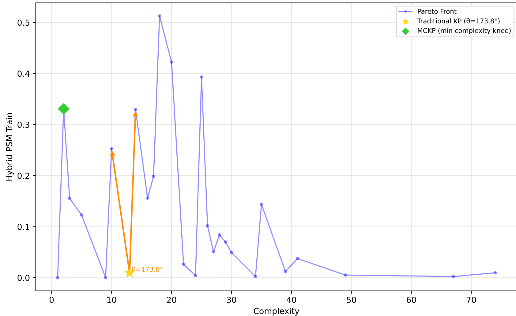
584_fri_c4_500_25 - Run 17 - MVP - Hybrid PSM Train \lambda_1=0.00, \bar{\lambda}_2=0.00, \bar{\lambda}_3=0.00 | Difficulty: 1.00 | Method: hmr
