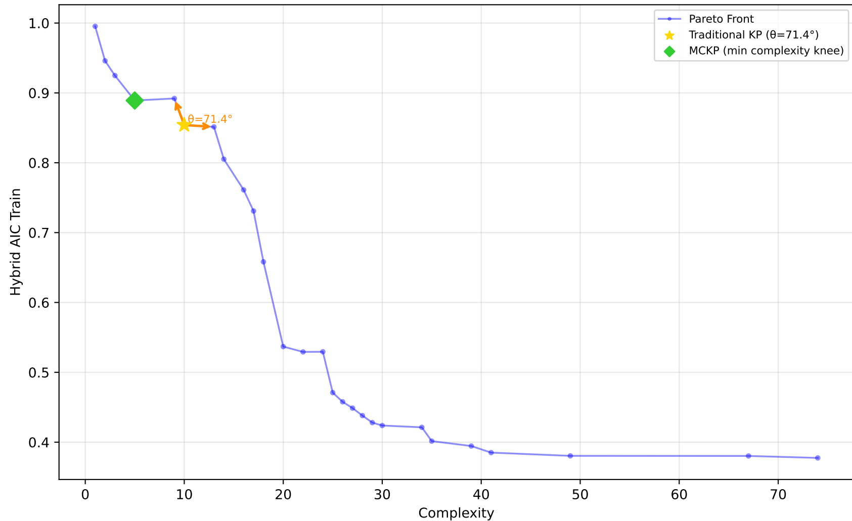
584_fri_c4_500_25 - Run 17 - SVP - Hybrid AIC Train \lambda_1=0.00, \lambda_2=0.00, \lambda_3=0.00 | Difficulty: 1.00 | Method: hmr
