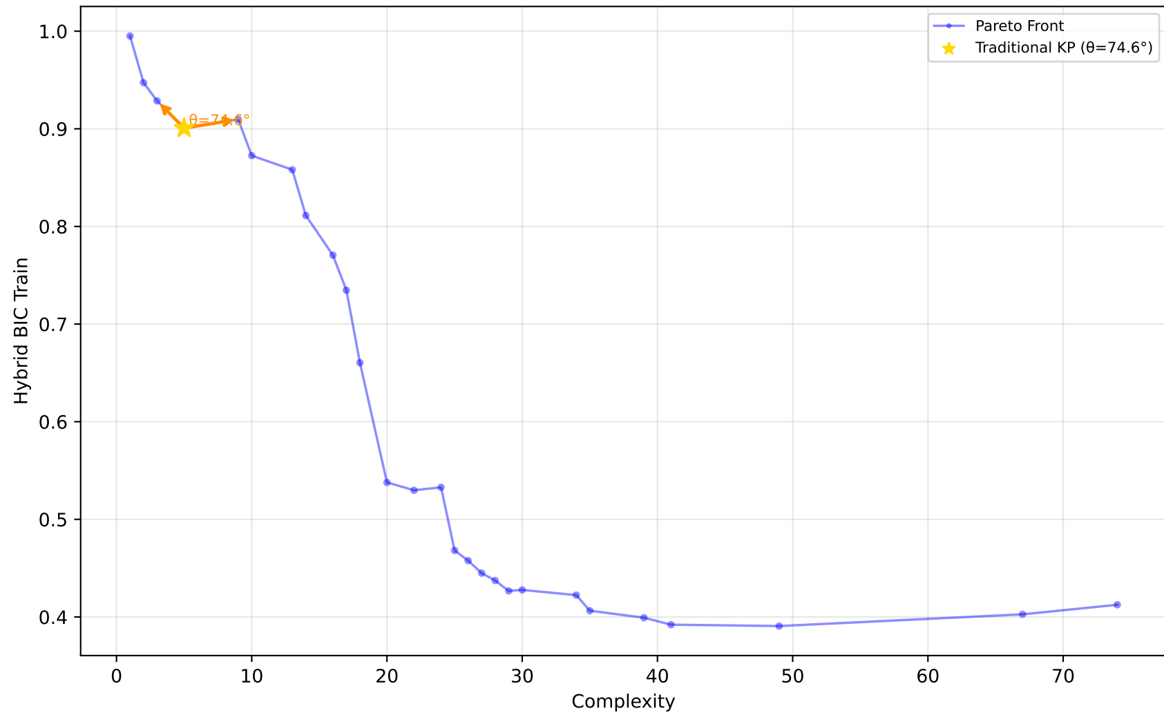
584_fri_c4_500_25 - Run 17 - SVP - Hybrid BIC Train \lambda_1=0.10, \lambda_2=0.40, \lambda_3=0.00 | Difficulty: 1.00 | Method: hmr
