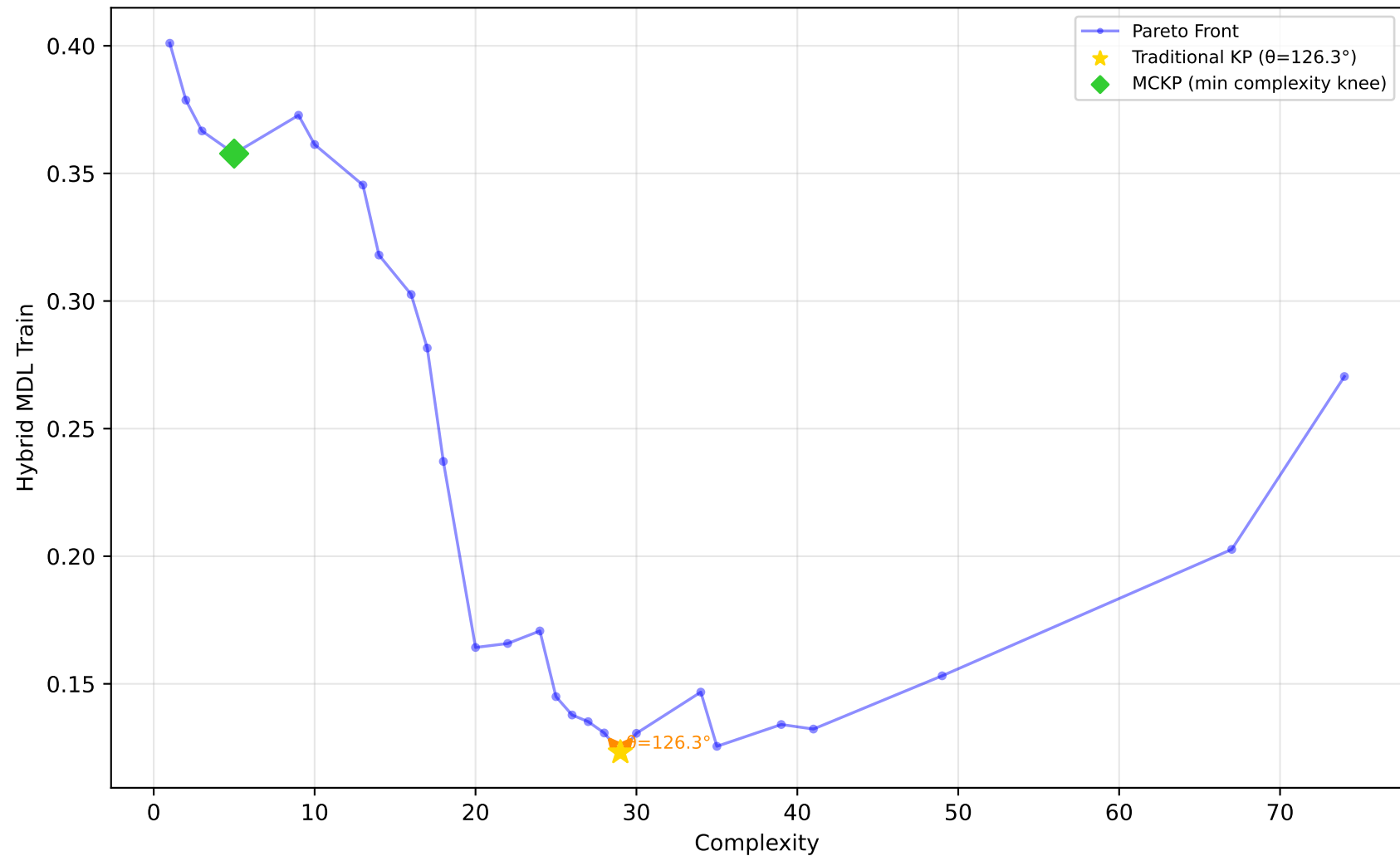
584_fri_c4_500_25 - Run 17 - SVP - Hybrid MDL Train \lambda_1=0.10, \lambda_2=0.40, \lambda_3=0.00 | Difficulty: 1.00 | Method: hmr
