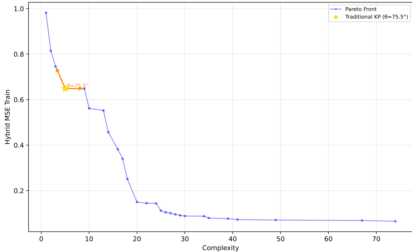
584_fri_c4_500_25 - Run 17 - SVP - Hybrid MSE Train \lambda_1=0.00, \lambda_2=0.00, \lambda_3=0.00 | Difficulty: 1.00 | Method: hmr
