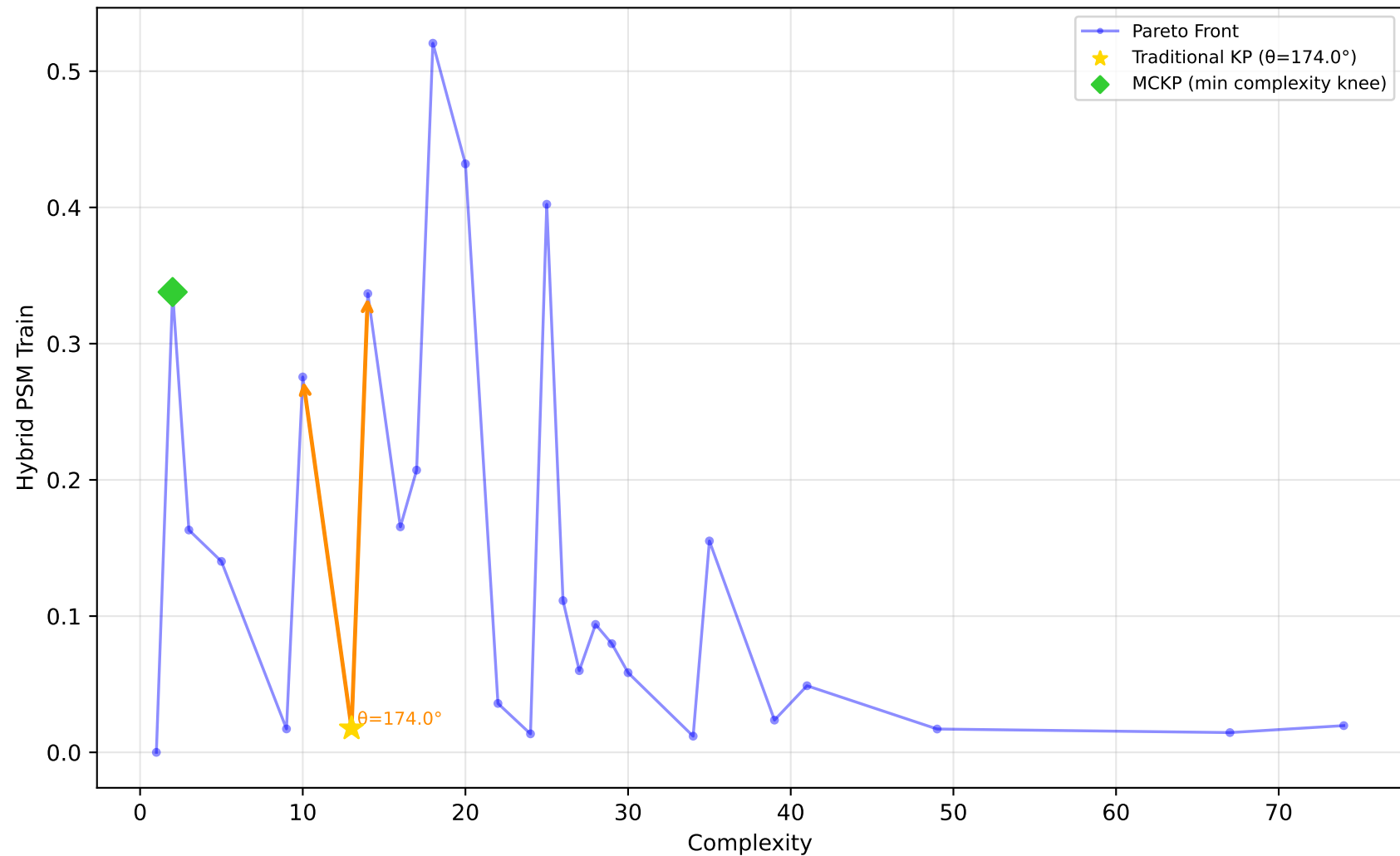
584_fri_c4_500_25 - Run 17 - SVP - Hybrid PSM Train \lambda_1=0.10, \lambda_2=0.40, \lambda_3=0.00 | Difficulty: 1.00 | Method: hmr
