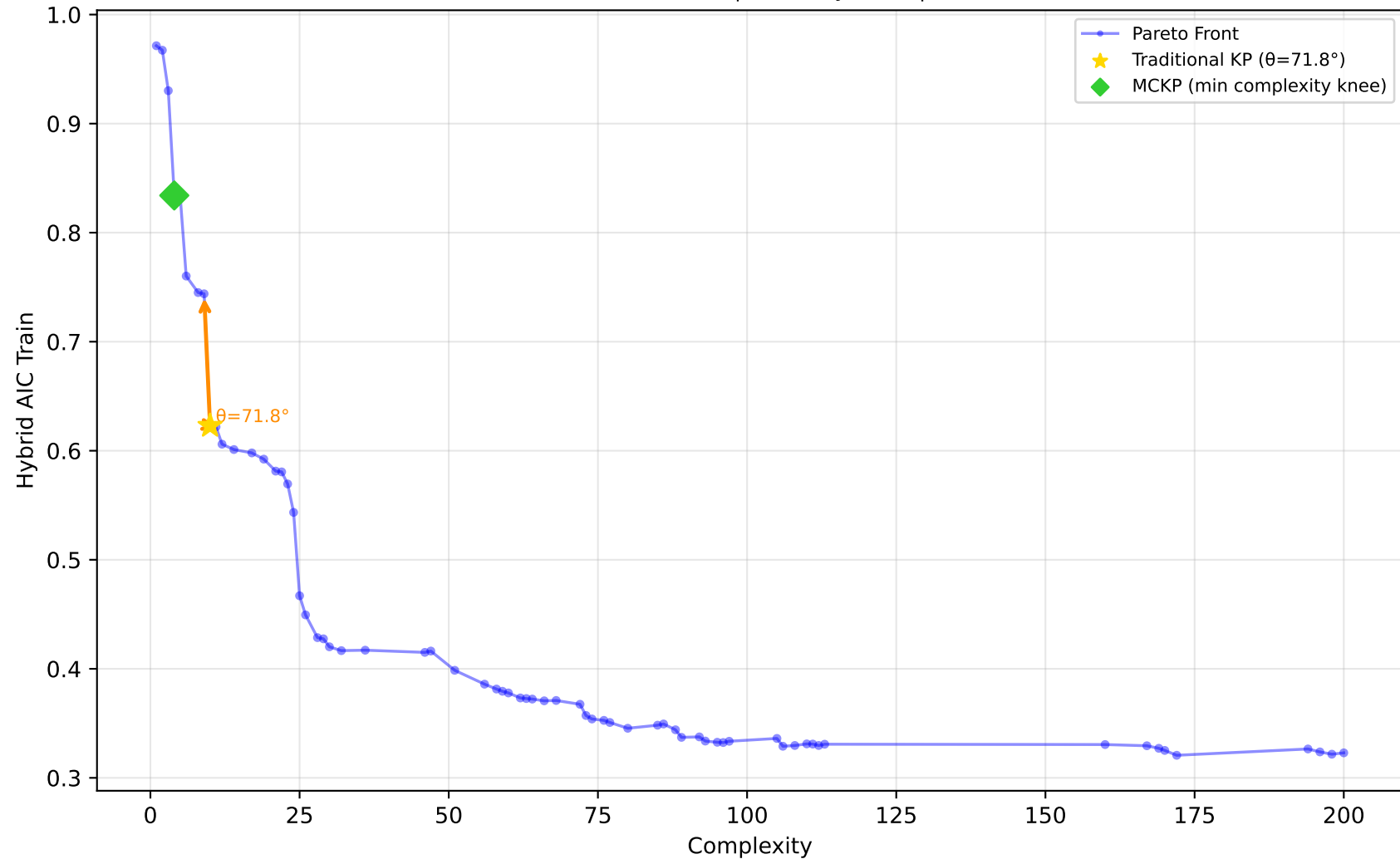
584_fri_c4_500_25 - Run 18 - MVP - Hybrid AIC Train \lambda_1=0.10, \lambda_2=0.00, \lambda_3=0.00 | Difficulty: 1.00 | Method: hmr
