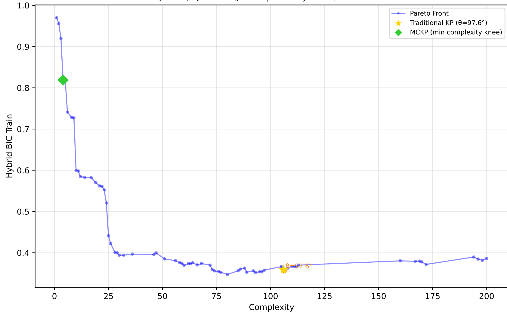
584_fri_c4_500_25 - Run 18 - MVP - Hybrid BIC Train \lambda_1=0.00, \lambda_2=0.00, \lambda_3=0.00 | Difficulty: 1.00 | Method: hmr
