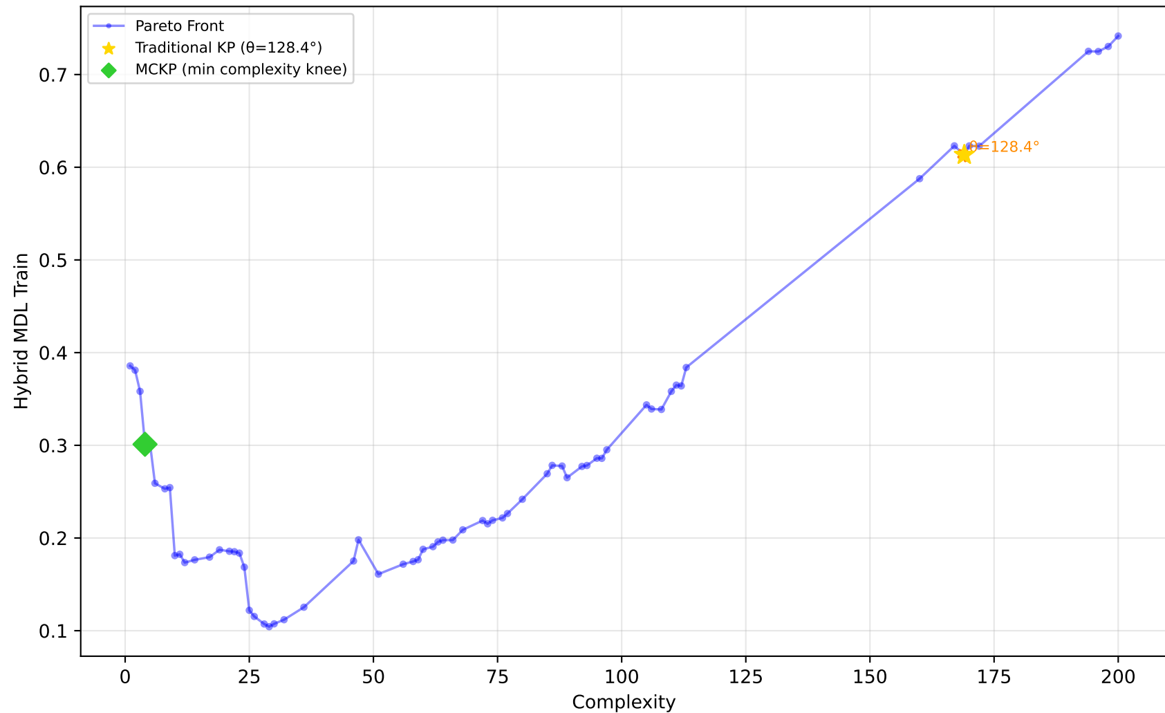
584_fri_c4_500_25 - Run 18 - MVP - Hybrid MDL Train \lambda_1=0.00, \bar{\lambda}_2=0.00, \lambda_3=0.00 | Difficulty: 1.00 | Method: hmr
