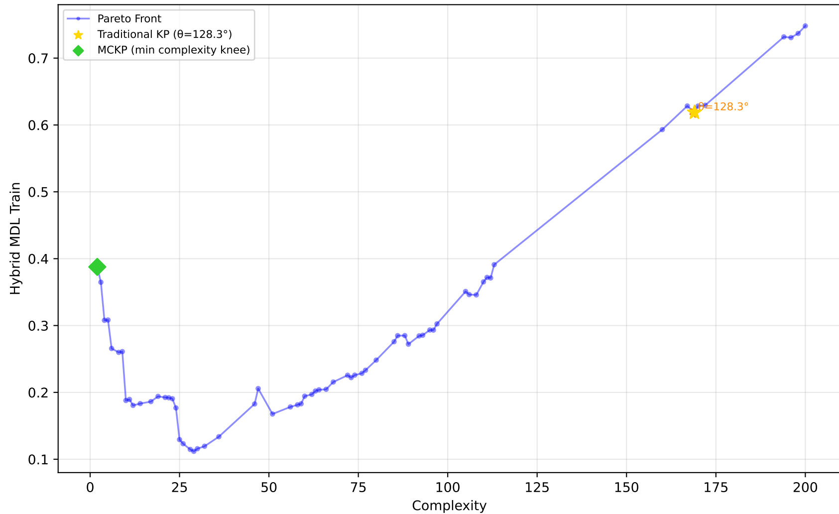
584_fri_c4_500_25 - Run 18 - MVP - Hybrid MDL Train \lambda_1=0.10, \bar{\lambda}_2=0.00, \bar{\lambda}_3=0.00 | Difficulty: 1.00 | Method: hmr
