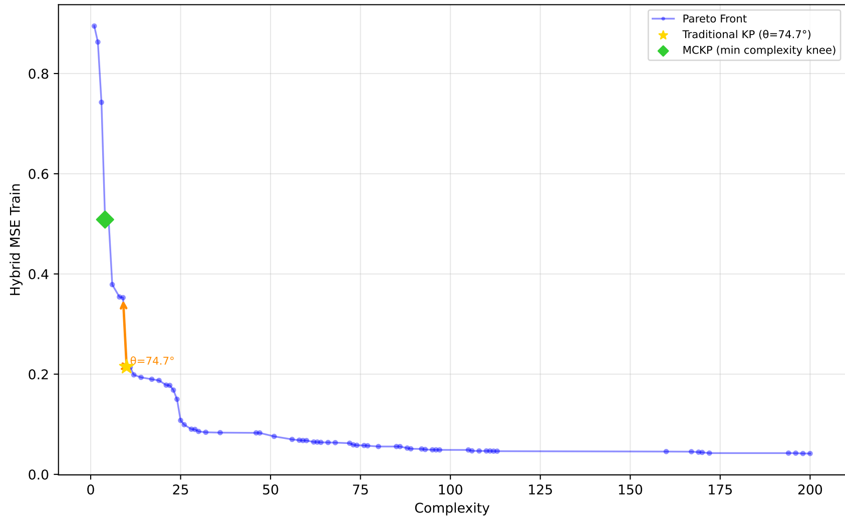
584_fri_c4_500_25 - Run 18 - MVP - Hybrid MSE Train \lambda_1=0.00, \lambda_2=0.00, \lambda_3=0.00 | Difficulty: 1.00 | Method: hmr
