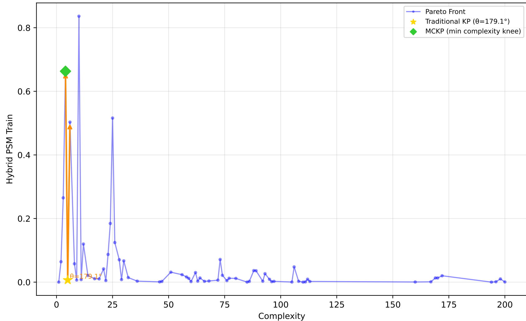
584_fri_c4_500_25 - Run 18 - MVP - Hybrid PSM Train \lambda_1=0.00, \bar{\lambda}_2=0.00, \bar{\lambda}_3=0.00 | Difficulty: 1.00 | Method: hmr
