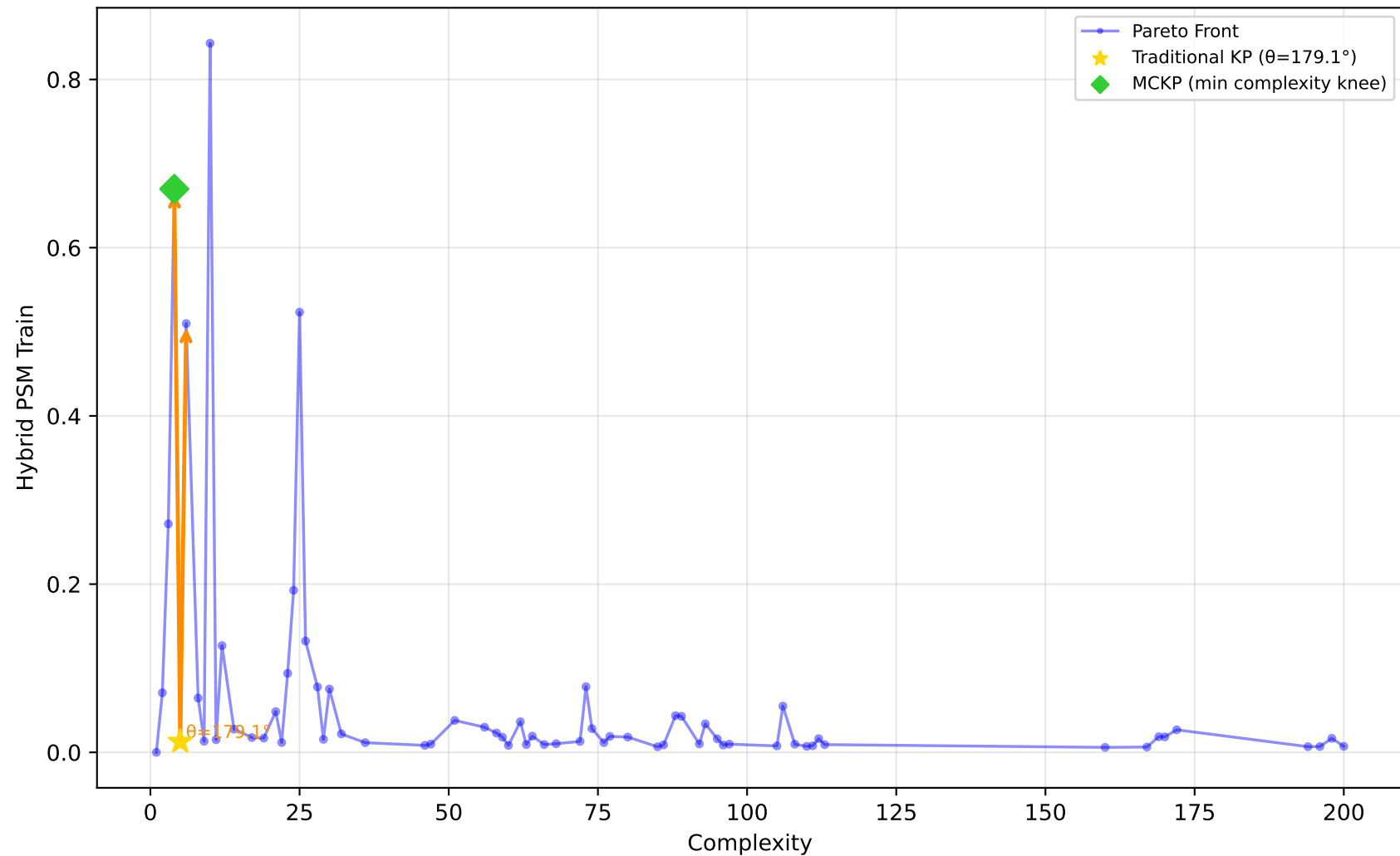
584_fri_c4_500_25 - Run 18 - MVP - Hybrid PSM Train \lambda_1=0.10, \bar{\lambda}_2=0.00, \bar{\lambda}_3=0.00 | Difficulty: 1.00 | Method: hmr
