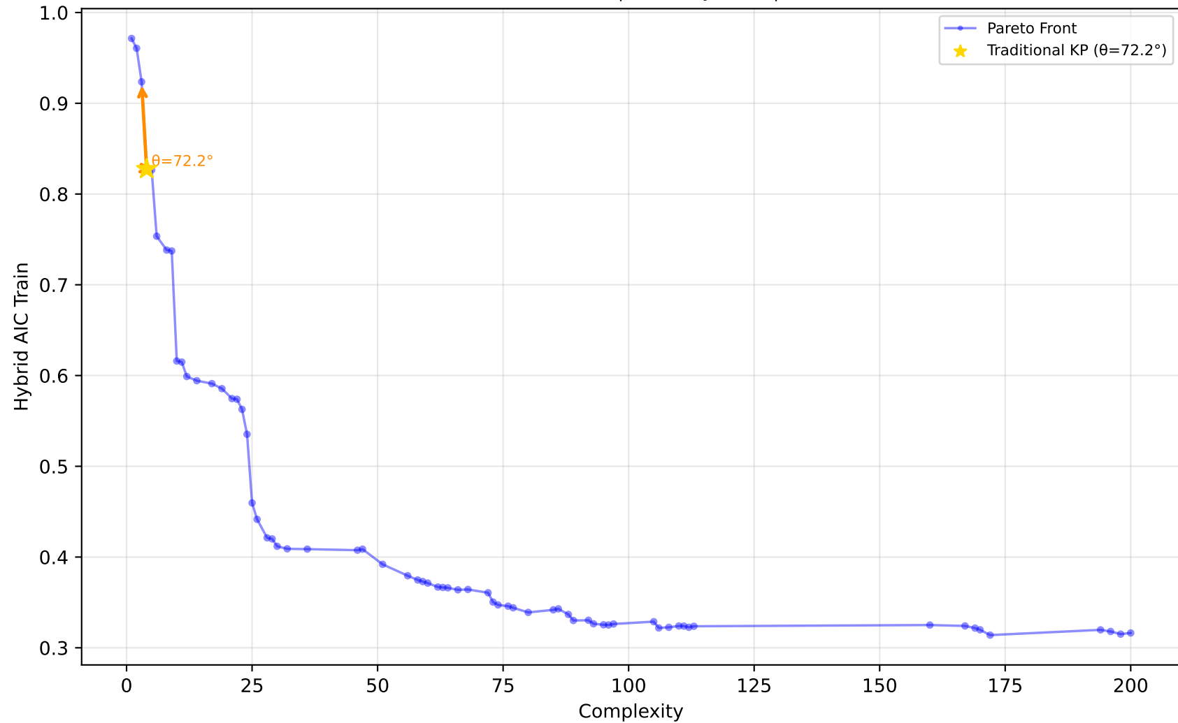
584_fri_c4_500_25 - Run 18 - SVP - Hybrid AIC Train \lambda_1=0.00, \lambda_2=0.00, \lambda_3=0.00 | Difficulty: 1.00 | Method: hmr
