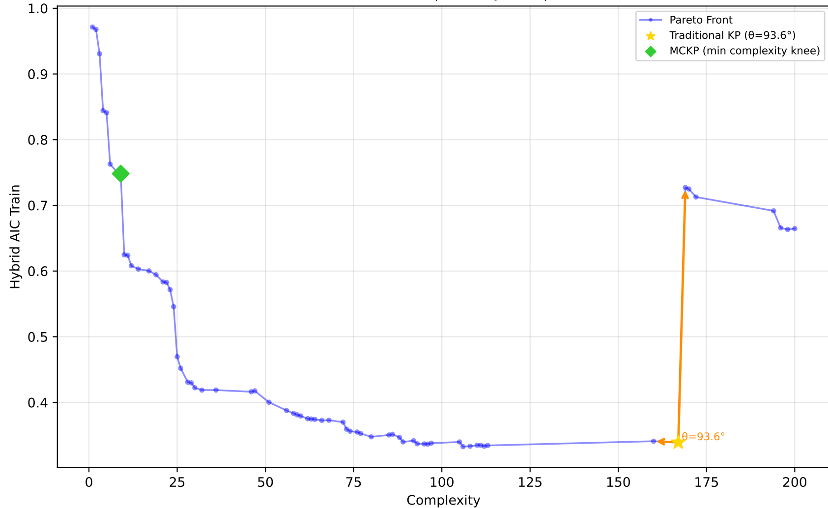
584_fri_c4_500_25 - Run 18 - SVP - Hybrid AIC Train \lambda_1=0.10, \lambda_2=0.40, \lambda_3=0.00 | Difficulty: 1.00 | Method: hmr
