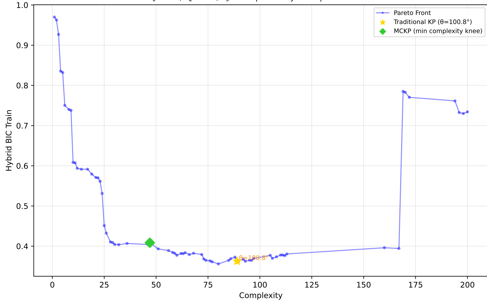
584_fri_c4_500_25 - Run 18 - SVP - Hybrid BIC Train \lambda_1=0.10, \lambda_2=0.40, \lambda_3=0.00 | Difficulty: 1.00 | Method: hmr
