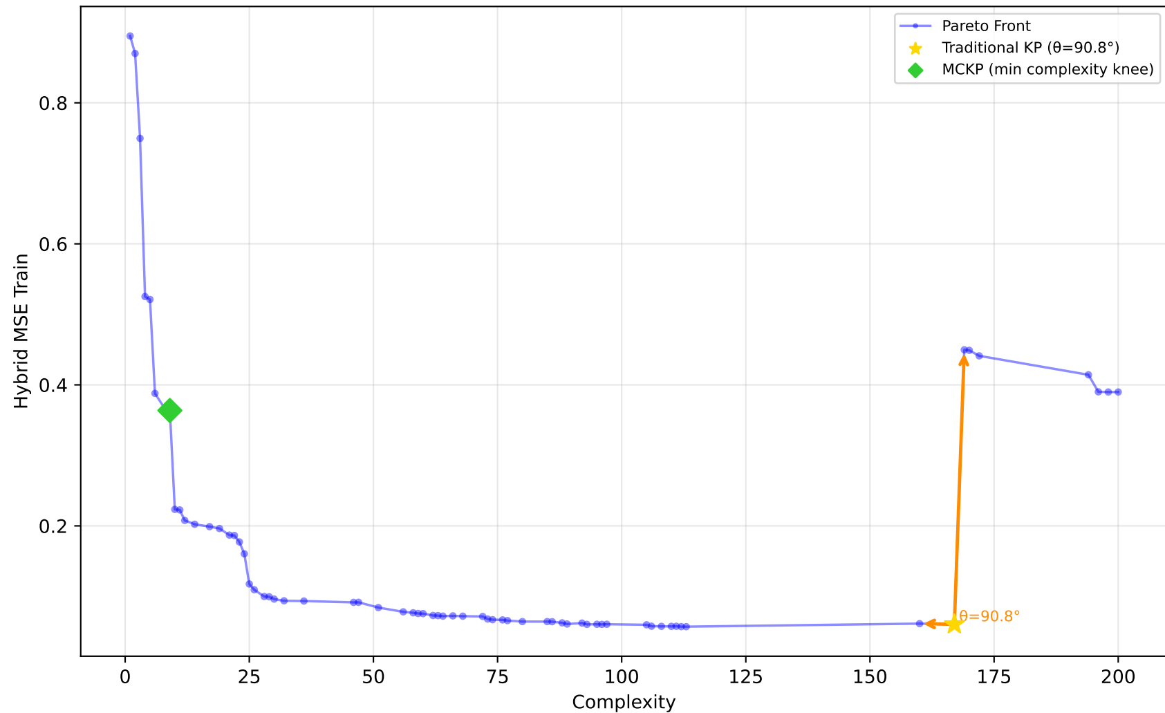
584_fri_c4_500_25 - Run 18 - SVP - Hybrid MSE Train \lambda_1=0.10, \lambda_2=0.40, \lambda_3=0.00 | Difficulty: 1.00 | Method: hmr
