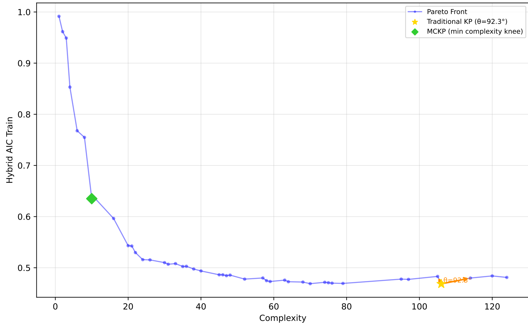
584_fri_c4_500_25 - Run 19 - MVP - Hybrid AIC Train \lambda_1=0.10, \lambda_2=0.00, \lambda_3=0.00 | Difficulty: 1.00 | Method: hmr
