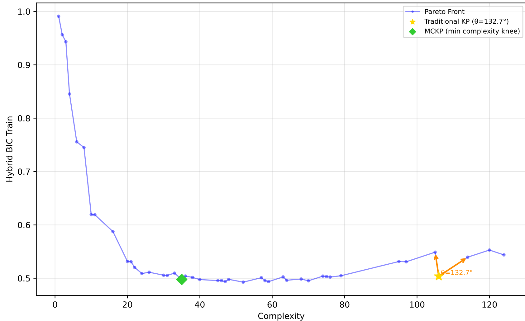
584_fri_c4_500_25 - Run 19 - MVP - Hybrid BIC Train \lambda_1=0.10, \lambda_2=0.00, \lambda_3=0.00 | Difficulty: 1.00 | Method: hmr
