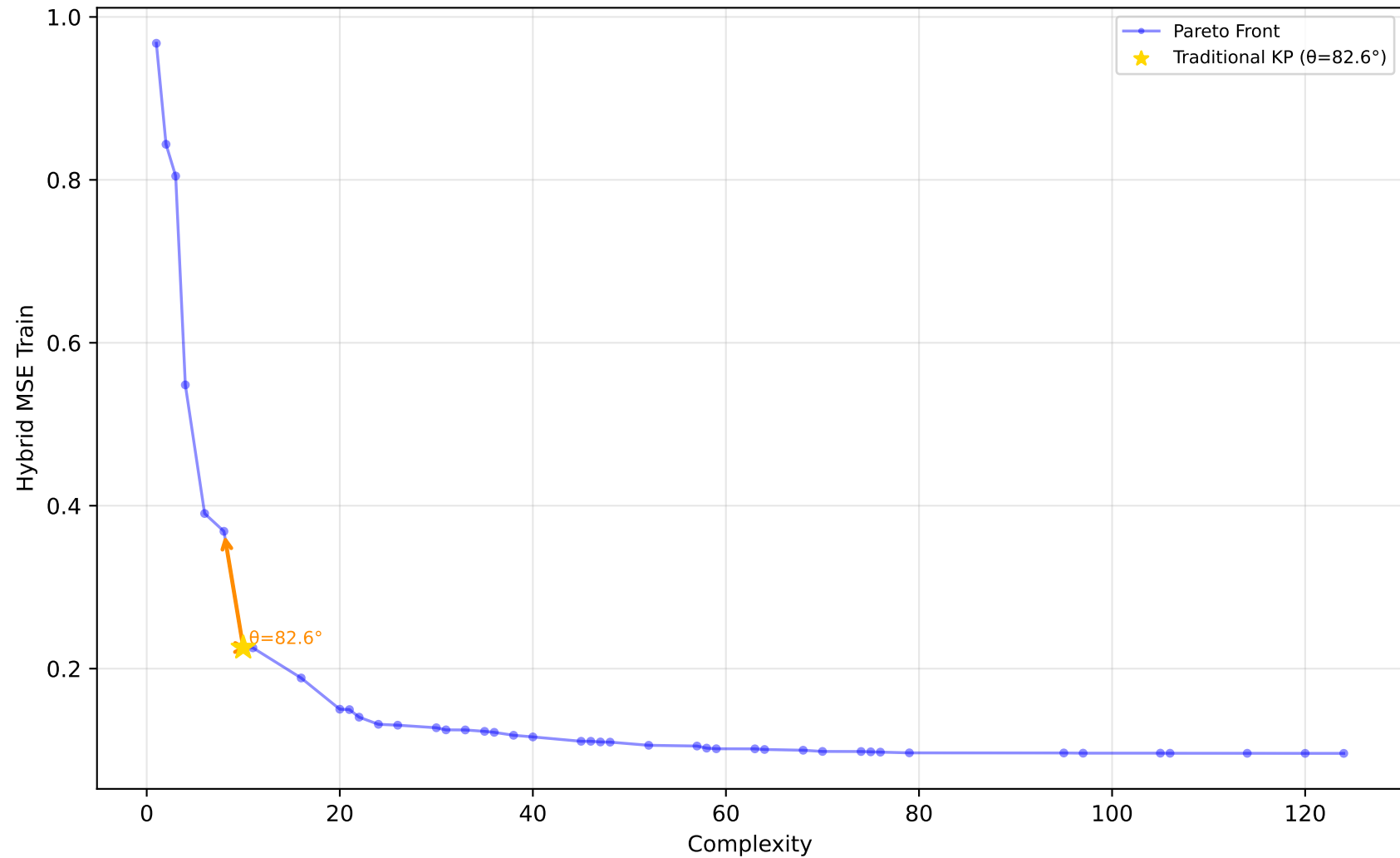
584_fri_c4_500_25 - Run 19 - MVP - Hybrid MSE Train \lambda_1=0.00, \bar{\lambda}_2=0.00, \bar{\lambda}_3=0.00 | Difficulty: 1.00 | Method: hmr
