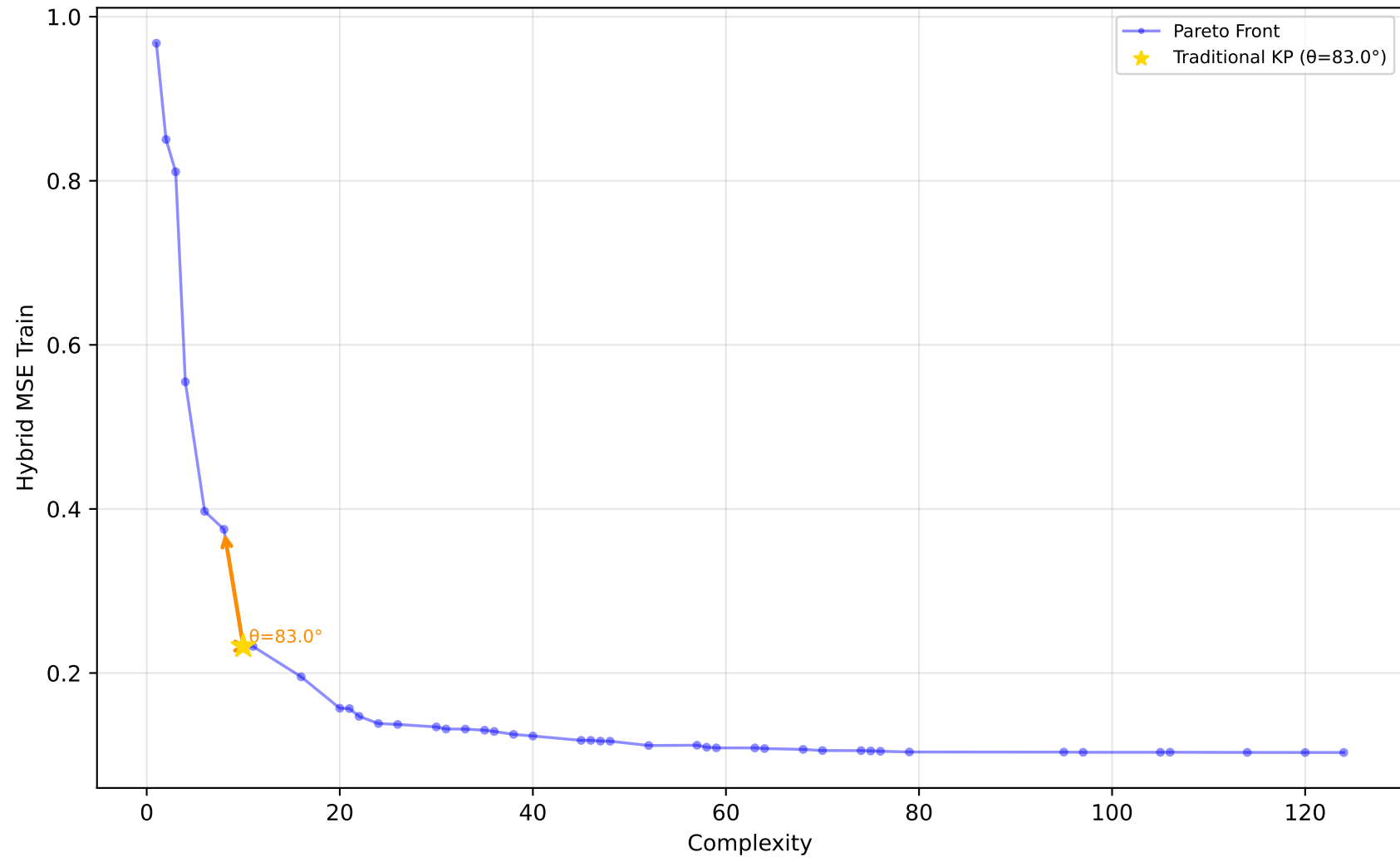
584_fri_c4_500_25 - Run 19 - MVP - Hybrid MSE Train \lambda_1=0.10, \bar{\lambda}_2=0.00, \bar{\lambda}_3=0.00 | Difficulty: 1.00 | Method: hmr
