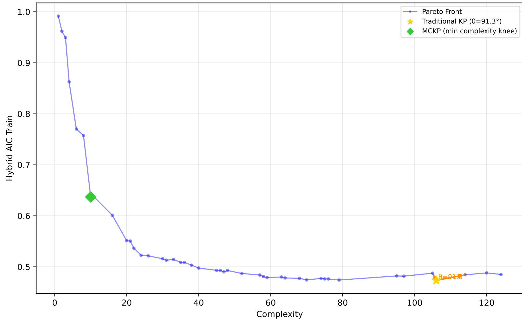
584_fri_c4_500_25 - Run 19 - SVP - Hybrid AIC Train \lambda_1=0.10, \lambda_2=0.40, \lambda_3=0.00 | Difficulty: 1.00 | Method: hmr
