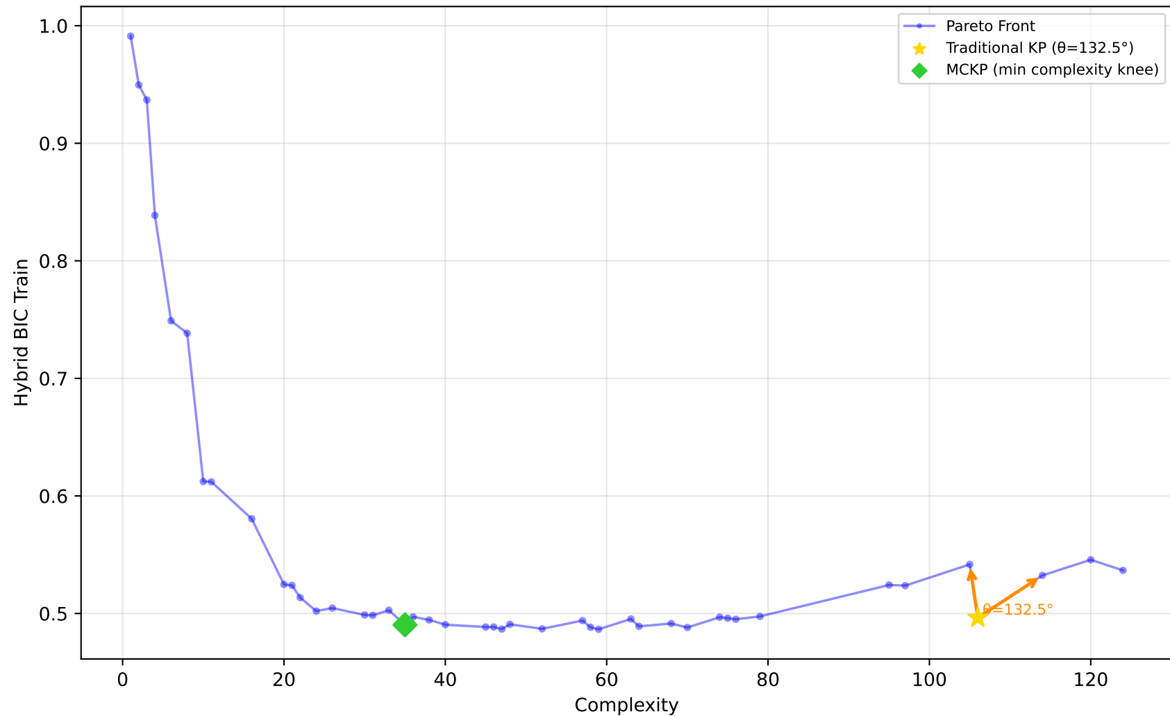
584_fri_c4_500_25 - Run 19 - SVP - Hybrid BIC Train \lambda_1=0.00, \lambda_2=0.00, \lambda_3=0.00 | Difficulty: 1.00 | Method: hmr
