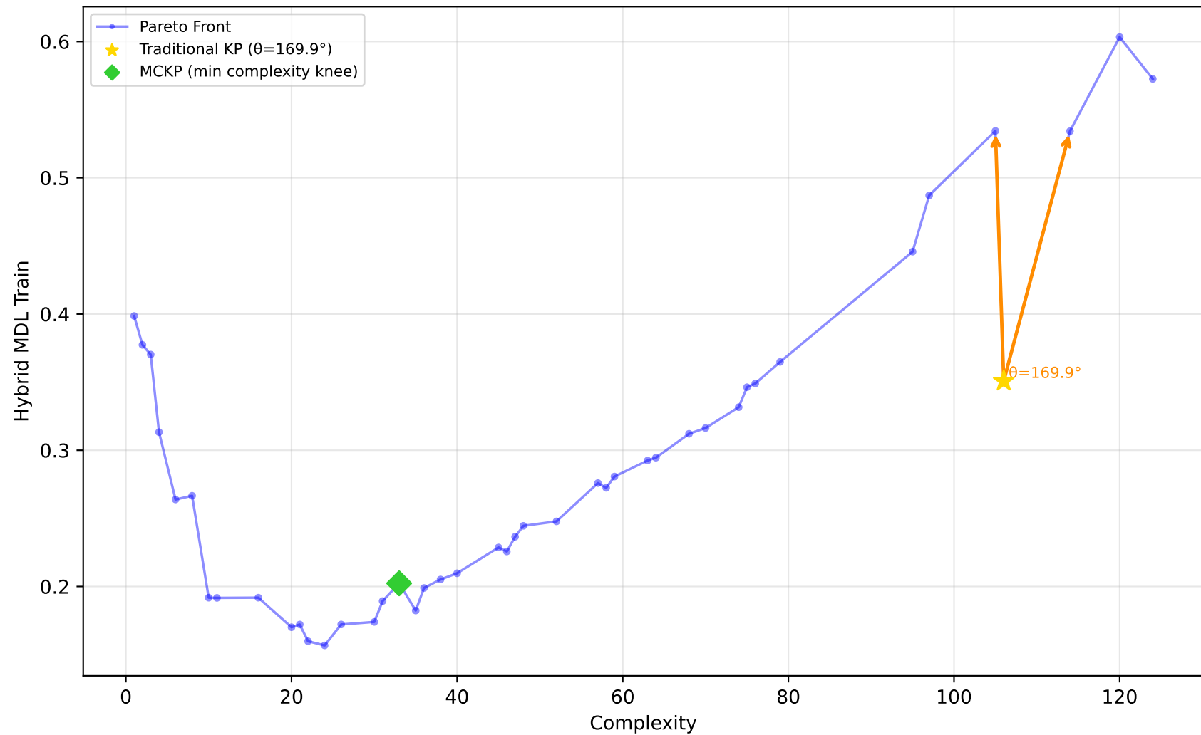
584_fri_c4_500_25 - Run 19 - SVP - Hybrid MDL Train \lambda_1=0.00, \lambda_2=0.00, \lambda_3=0.00 | Difficulty: 1.00 | Method: hmr
