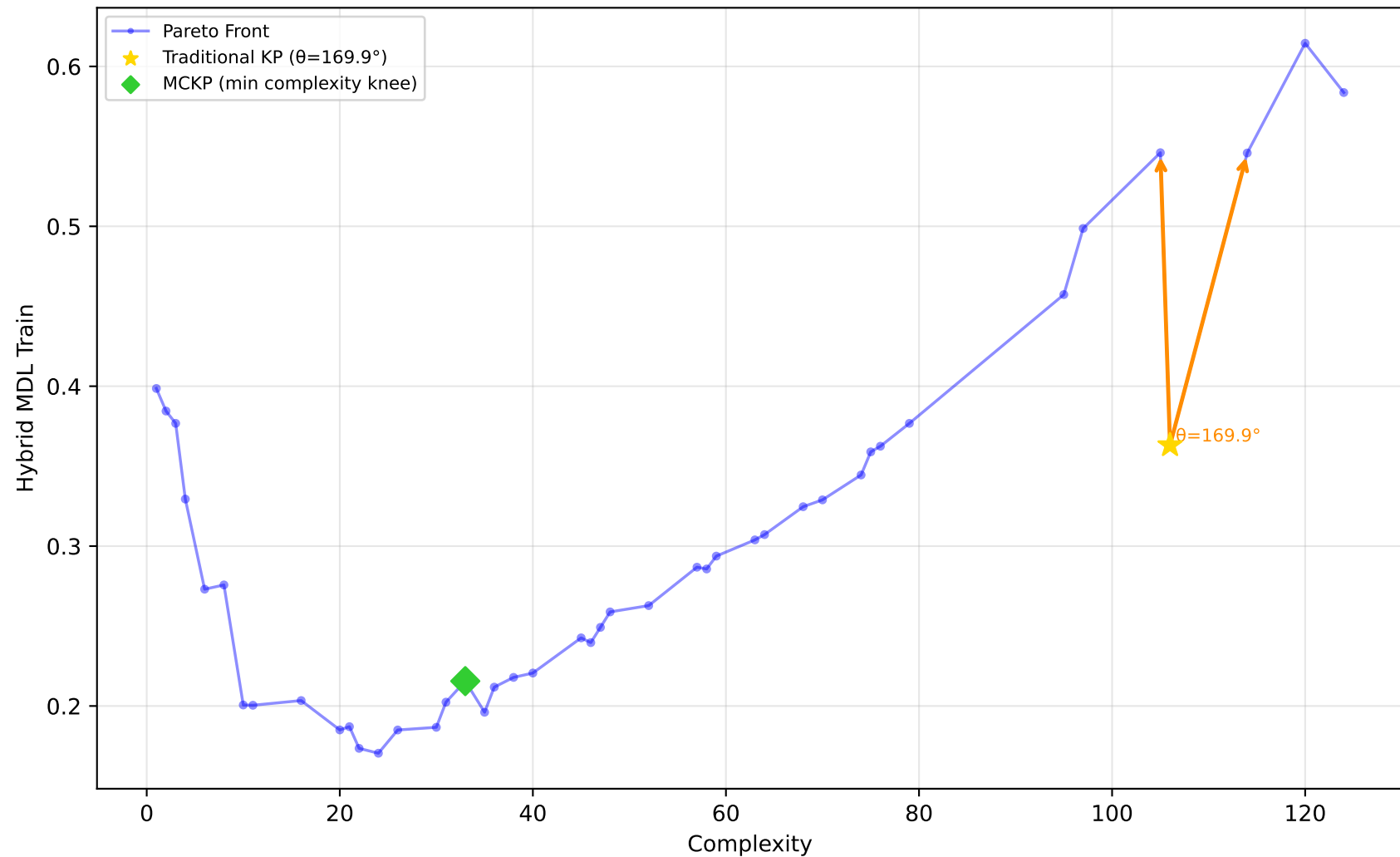
584_fri_c4_500_25 - Run 19 - SVP - Hybrid MDL Train \lambda_1=0.10, \lambda_2=0.40, \lambda_3=0.00 | Difficulty: 1.00 | Method: hmr
