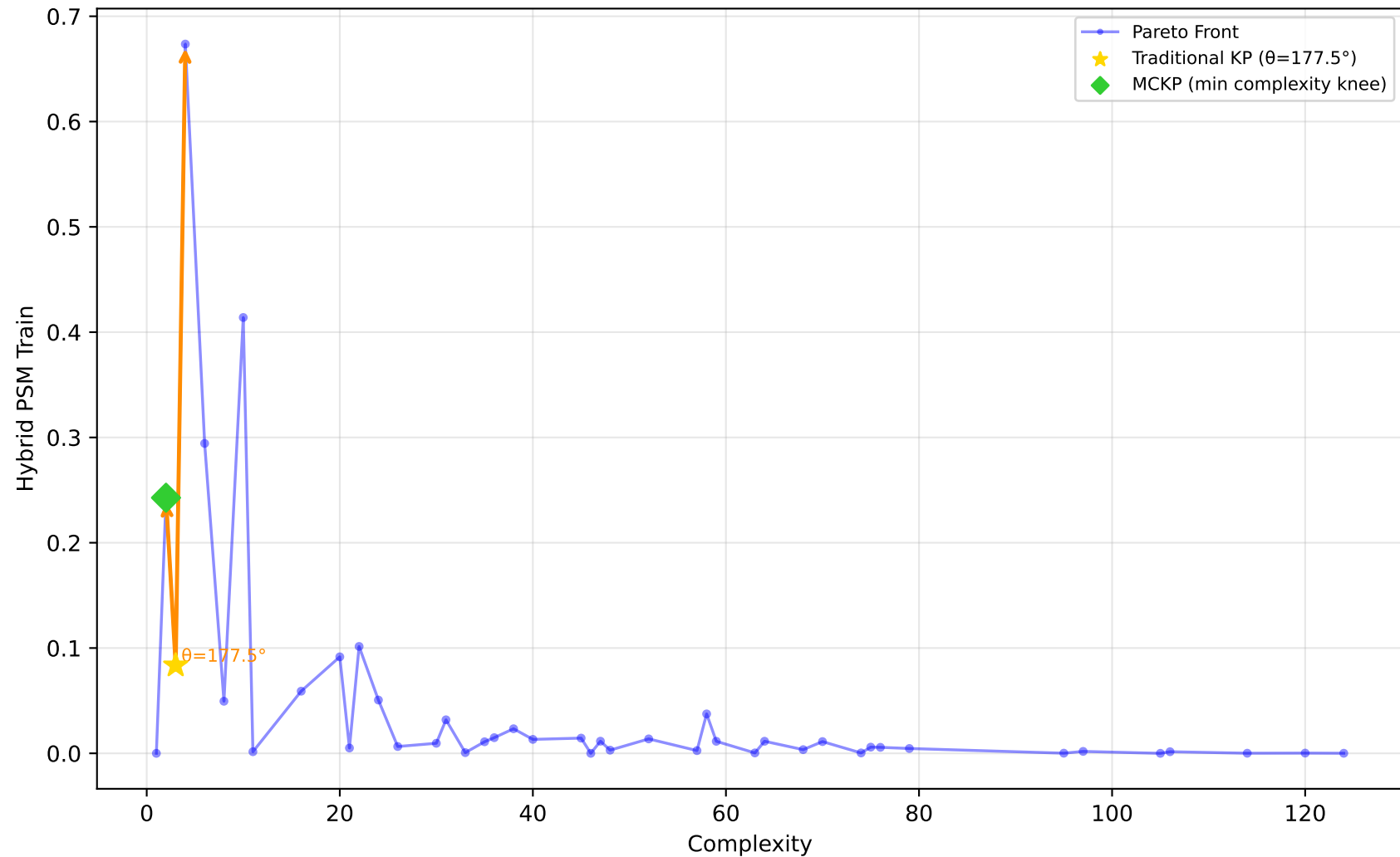
584_fri_c4_500_25 - Run 19 - SVP - Hybrid PSM Train \lambda_1=0.00, \lambda_2=0.00, \lambda_3=0.00 | Difficulty: 1.00 | Method: hmr
