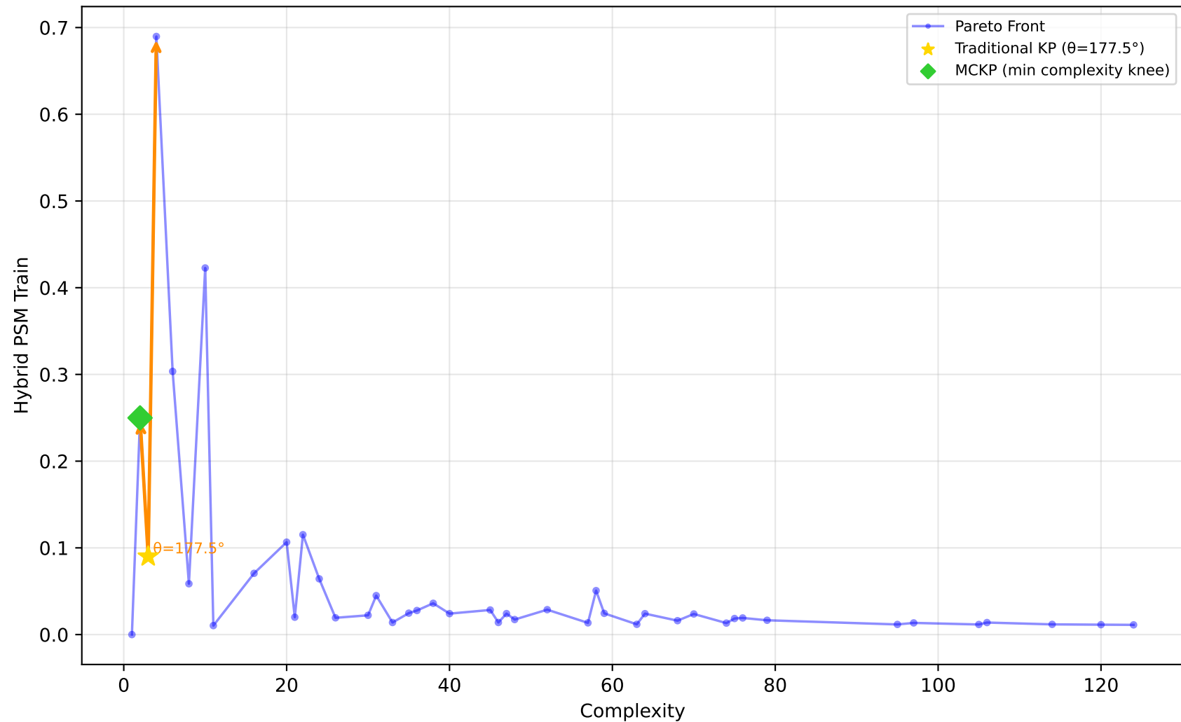
584_fri_c4_500_25 - Run 19 - SVP - Hybrid PSM Train \lambda_1=0.10, \lambda_2=0.40, \lambda_3=0.00 | Difficulty: 1.00 | Method: hmr
