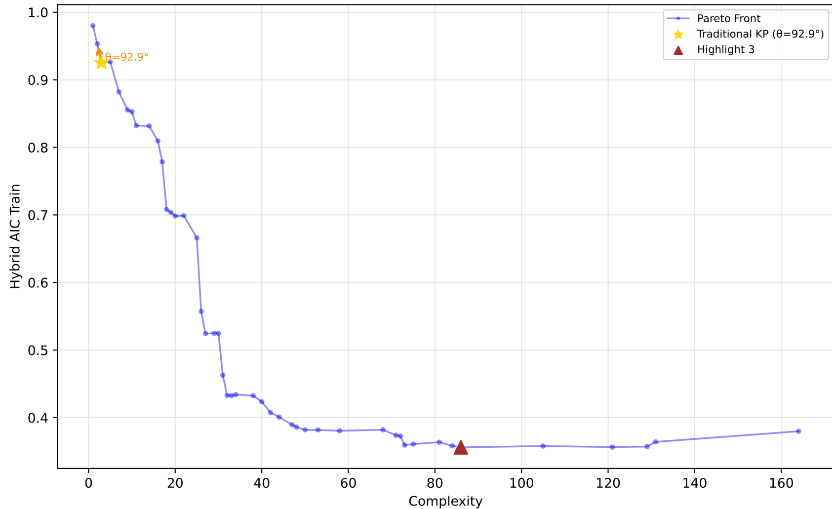
584_fri_c4_500_25 - Run 1 - MVP - Hybrid AIC Train \lambda_1=0.00, \lambda_2=0.00, \lambda_3=0.00 | Difficulty: 1.00 | Method: hmr
