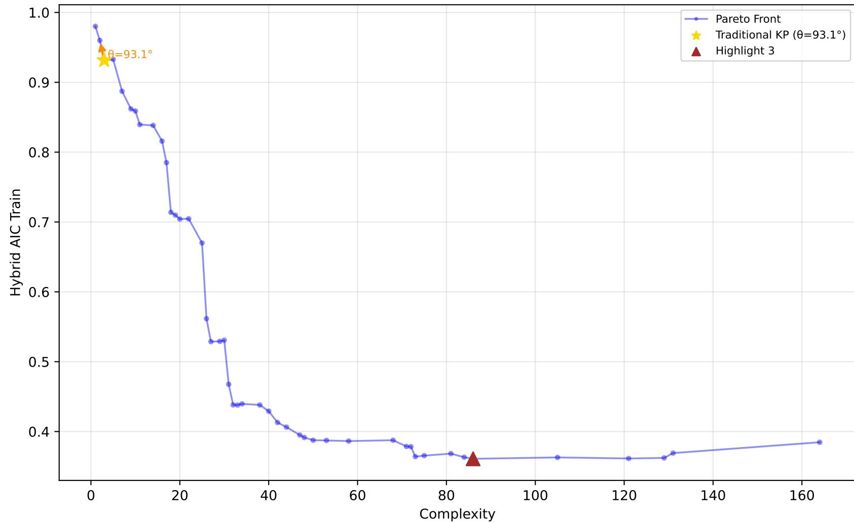
584_fri_c4_500_25 - Run 1 - MVP - Hybrid AIC Train \lambda_1=0.10, \lambda_2=0.00, \lambda_3=0.00 | Difficulty: 1.00 | Method: hmr
