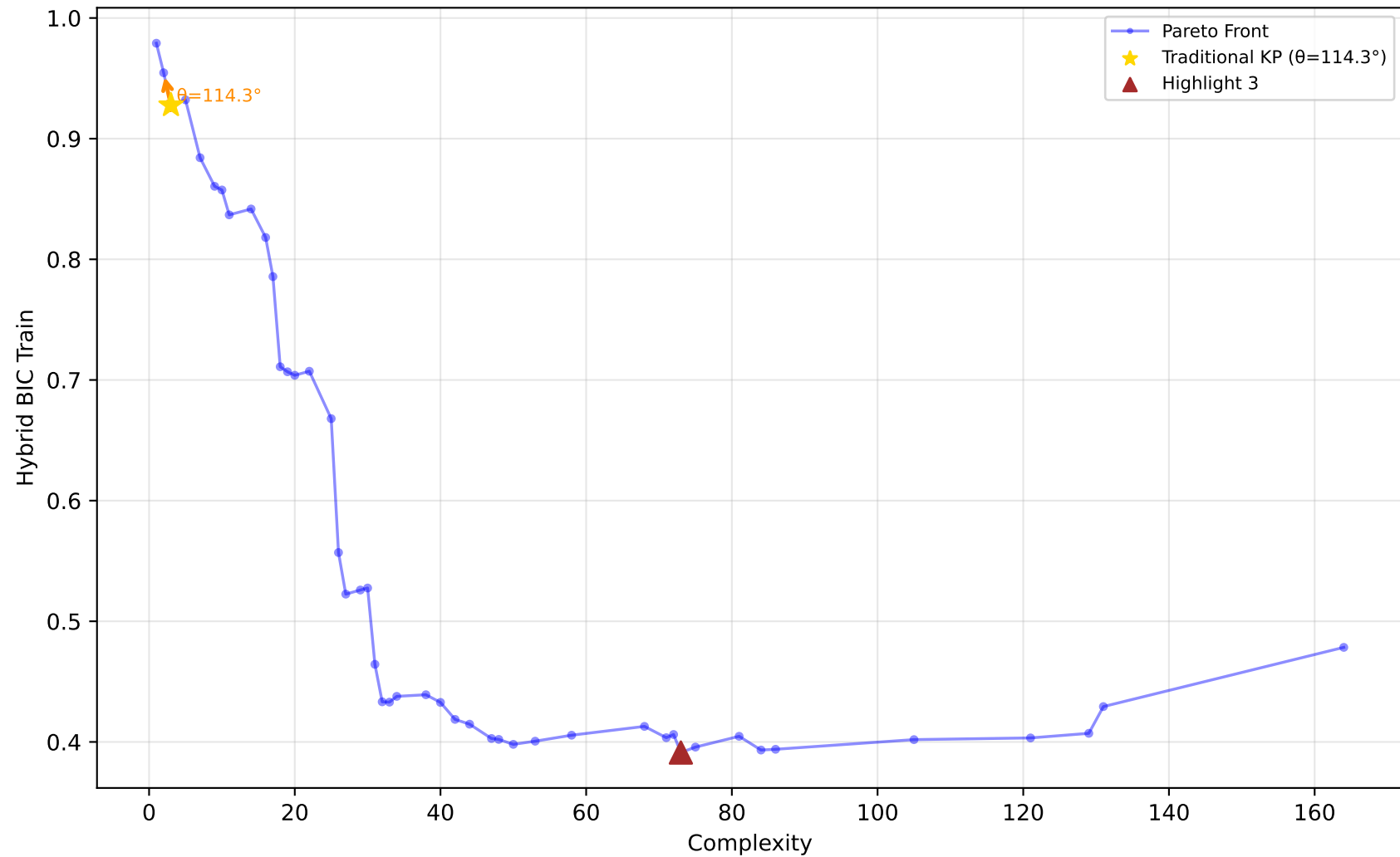
584_fri_c4_500_25 - Run 1 - MVP - Hybrid BIC Train \lambda_1=0.10, \lambda_2=0.00, \lambda_3=0.00 | Difficulty: 1.00 | Method: hmr
