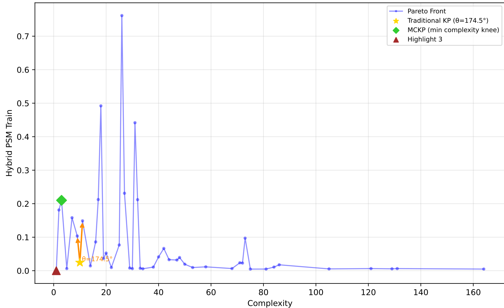
584_fri_c4_500_25 - Run 1 - MVP - Hybrid PSM Train \lambda_1=0.10, \lambda_2=0.00, \lambda_3=0.00 | Difficulty: 1.00 | Method: hmr
