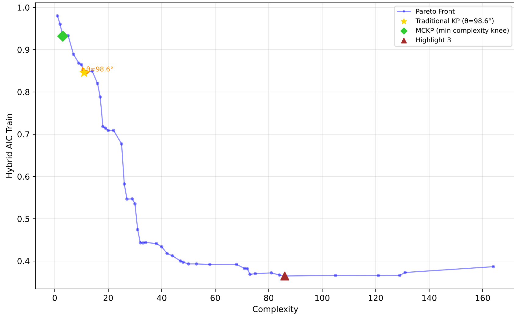
584_fri_c4_500_25 - Run 1 - SVP - Hybrid AIC Train \lambda_1=0.10, \lambda_2=0.40, \lambda_3=0.00 | Difficulty: 1.00 | Method: hmr
