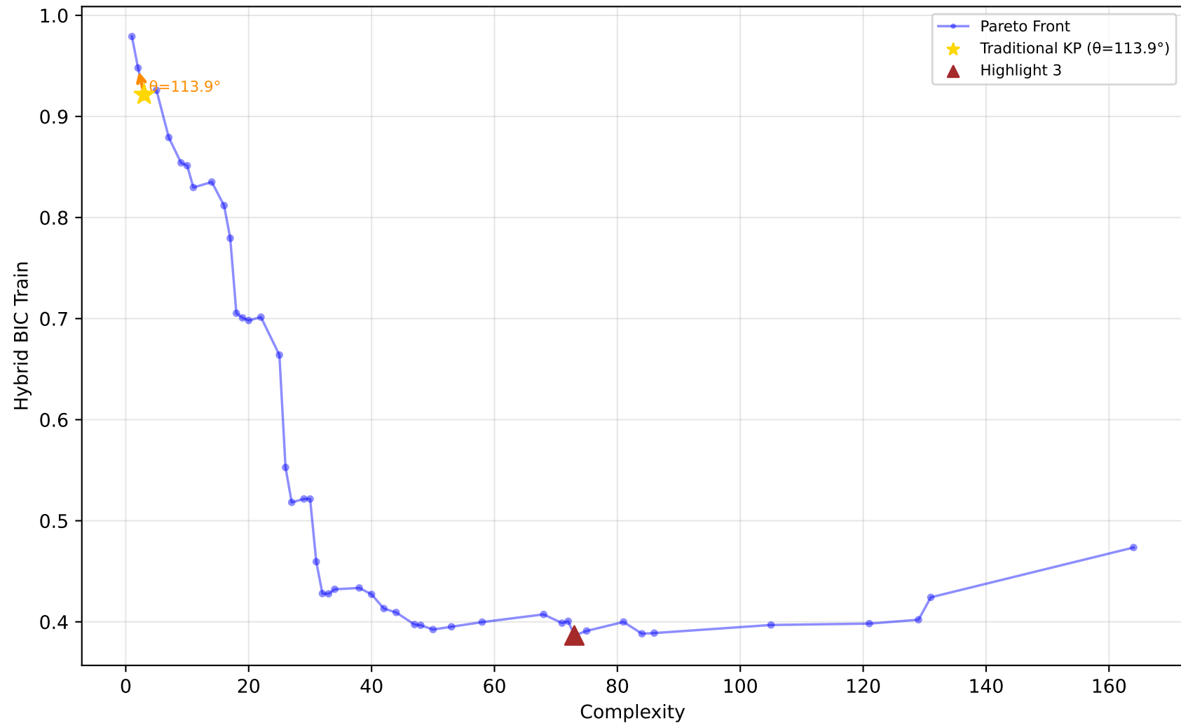
584_fri_c4_500_25 - Run 1 - SVP - Hybrid BIC Train \lambda_1=0.00, \lambda_2=0.00, \lambda_3=0.00 | Difficulty: 1.00 | Method: hmr
