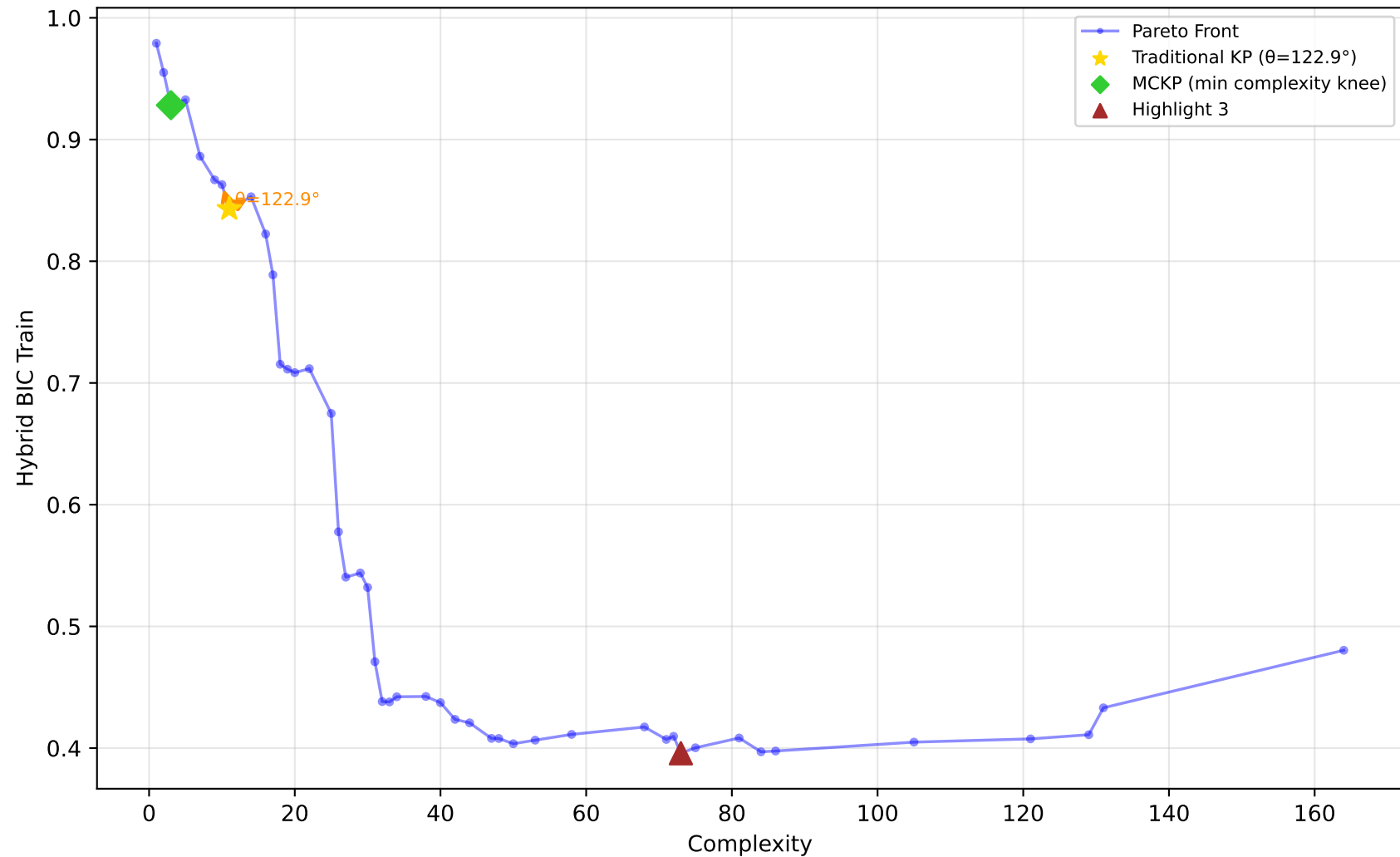
584_fri_c4_500_25 - Run 1 - SVP - Hybrid BIC Train \lambda_1=0.10, \lambda_2=0.40, \lambda_3=0.00 | Difficulty: 1.00 | Method: hmr
