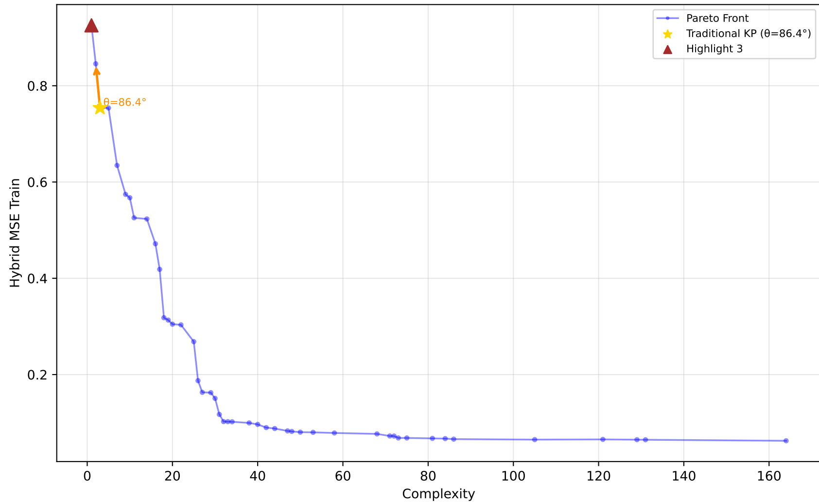
584_fri_c4_500_25 - Run 1 - SVP - Hybrid MSE Train \lambda_1=0.10, \lambda_2=0.40, \lambda_3=0.00 | Difficulty: 1.00 | Method: hmr
